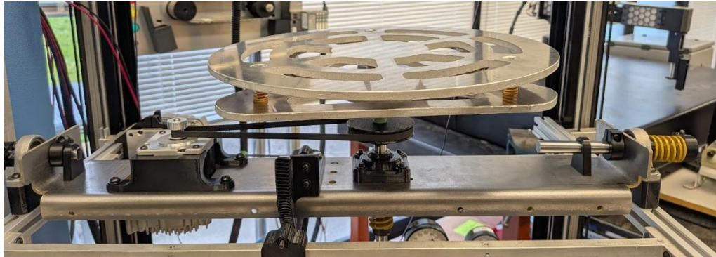
Figure 10 – Implemented Printer bed and Yaw Axis
