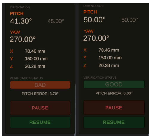
Figure 21 – Unity Verification Status Banner (BAD (left) and GOOD (right))
