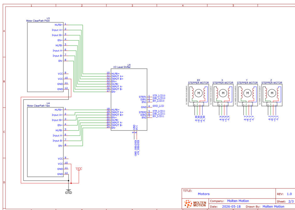
Figure F1 - Angle Monitoring System Electrical Schematic
