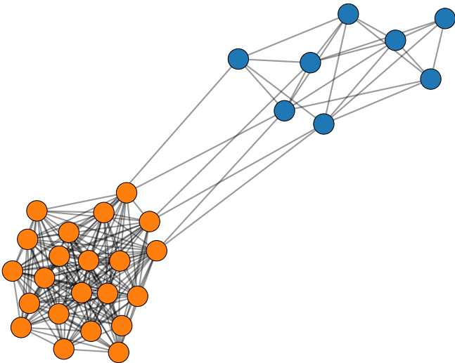
Graph 3 (206 edges)
