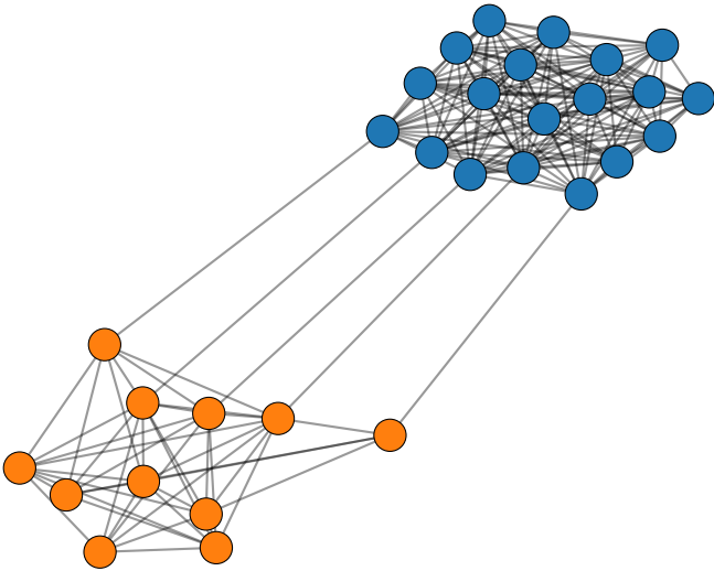
Graph 3 (206 edges)
