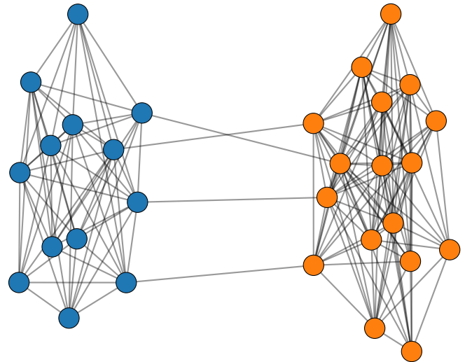
Graph 4 (170 edges)
