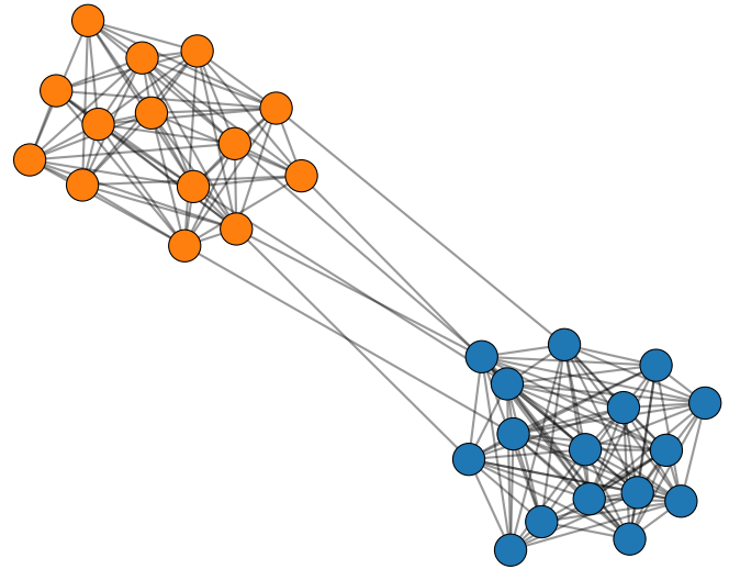
Graph 4 (170 edges)
