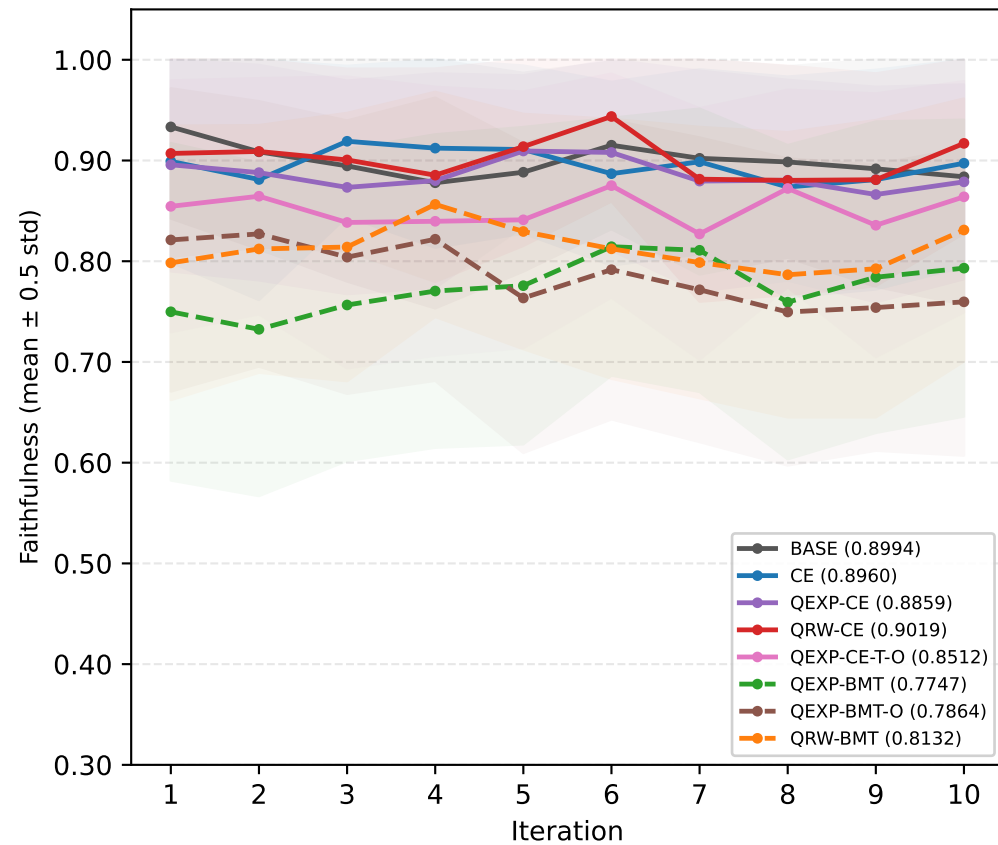
Faithfulness
