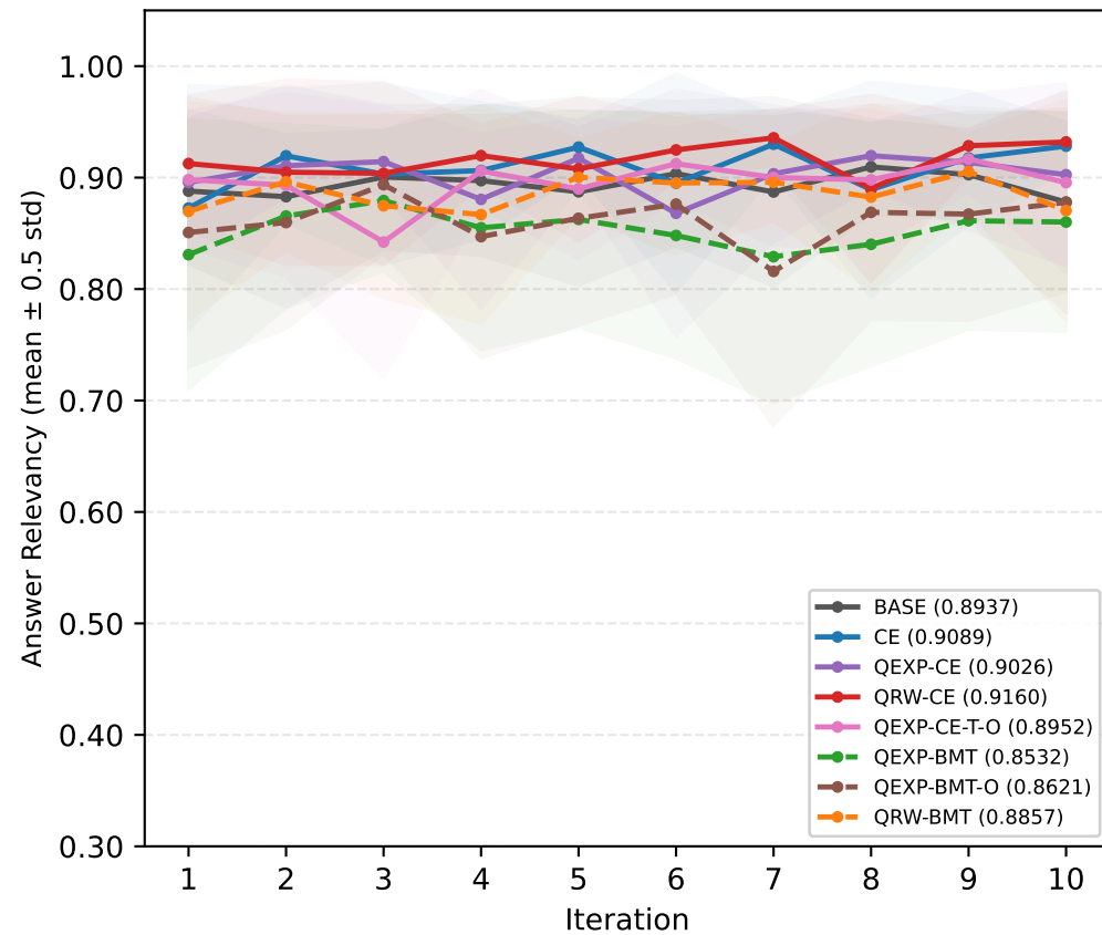
Answer Relevancy
