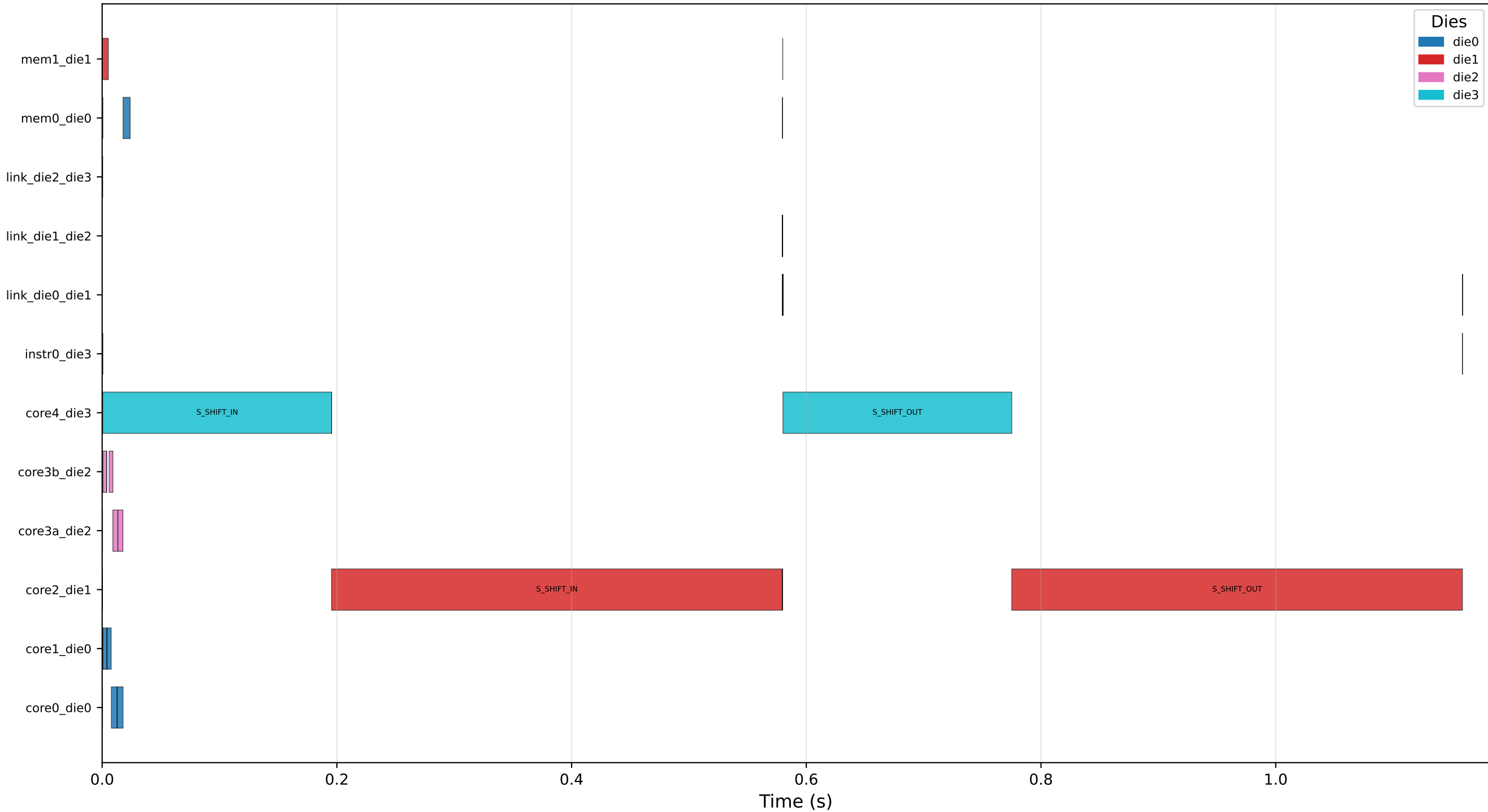
Figure 10: Gantt Chart -- v4_4die_3d_stack / bist_fpp_thermal / CP-SAT
