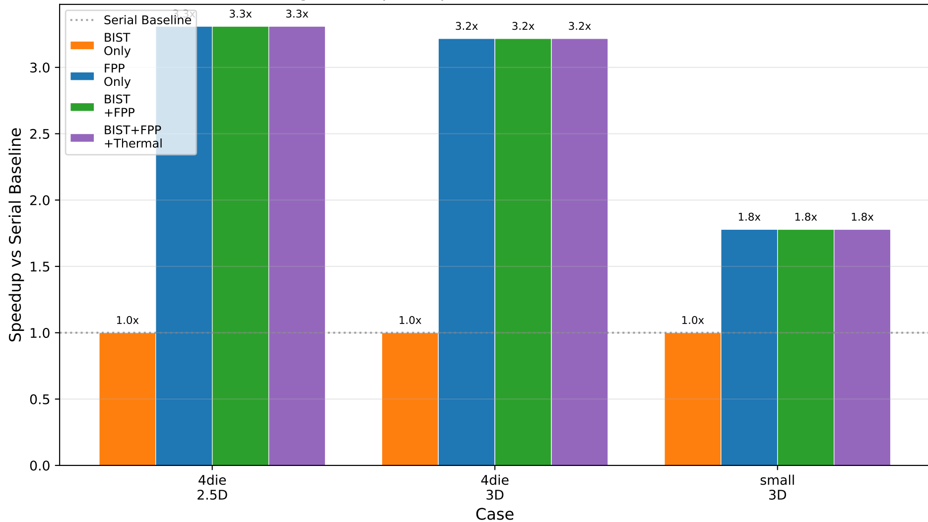
Figure 2: Speedup vs Serial Baseline (CP-SAT)
