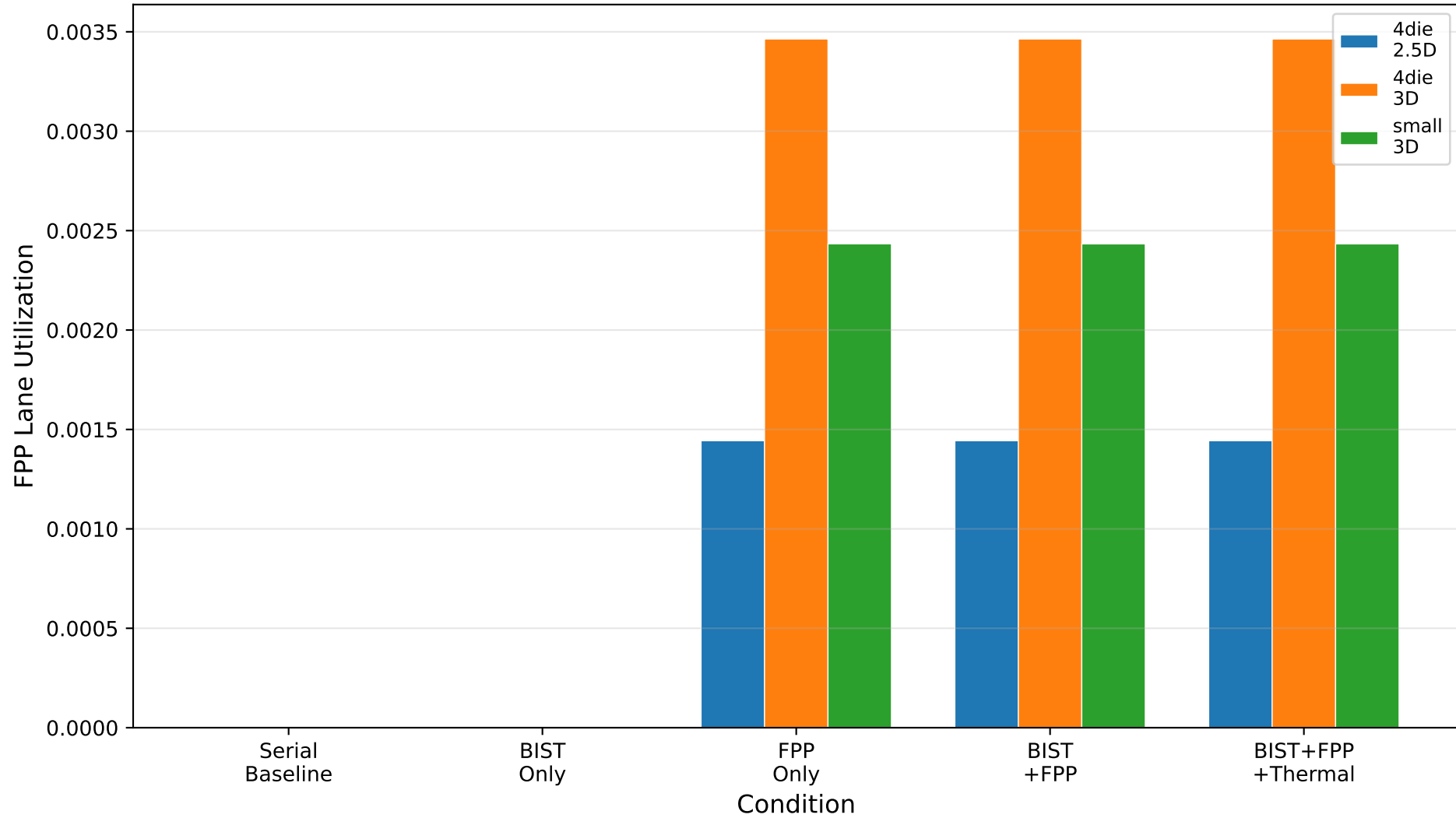
Figure 4: FPP Utilization Across Conditions (CP-SAT)
