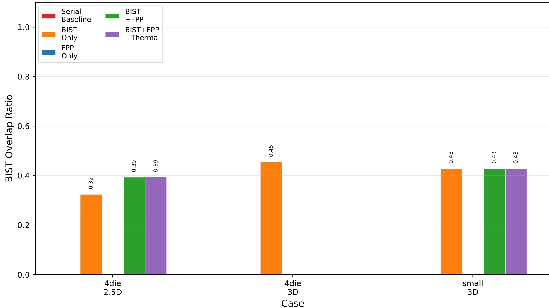
Figure 5: BIST Overlap Ratio (CP-SAT)
