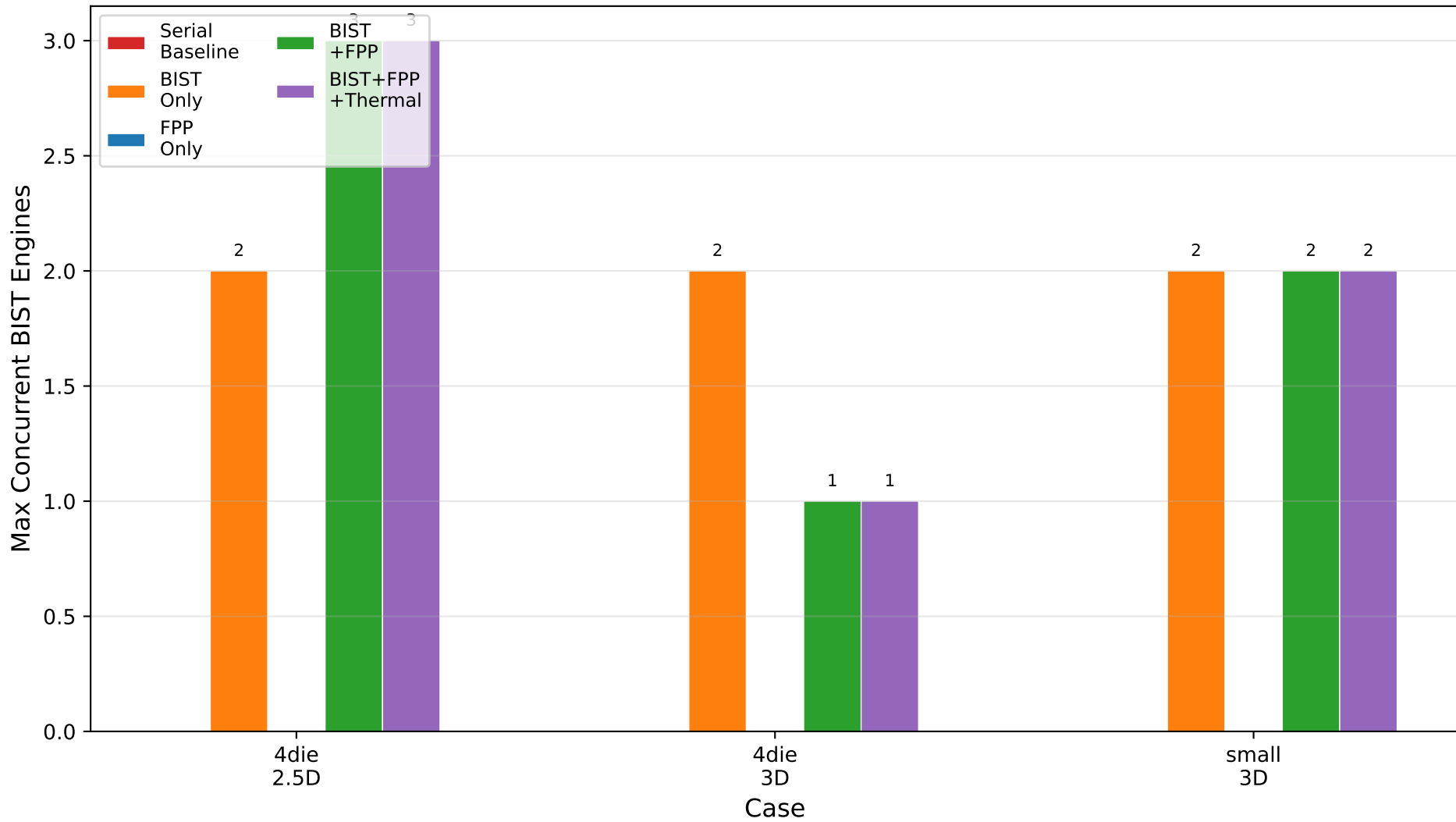
Figure 6: Max Concurrent BIST Engines (CP-SAT)
