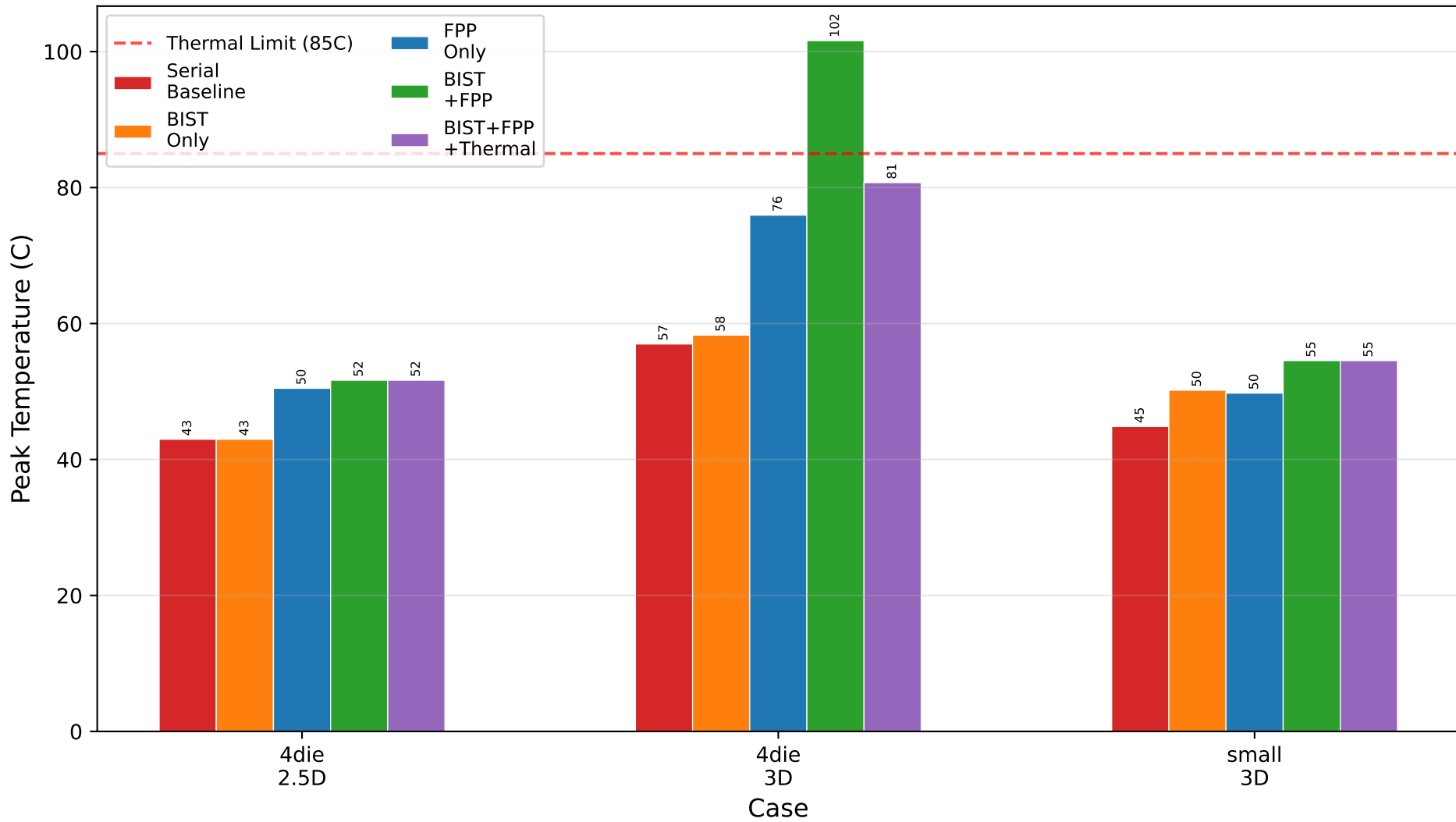
Figure 7: Peak Temperature Across Conditions (CP-SAT)
