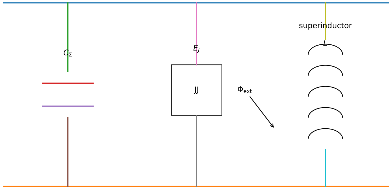
Fluxonium circuit
