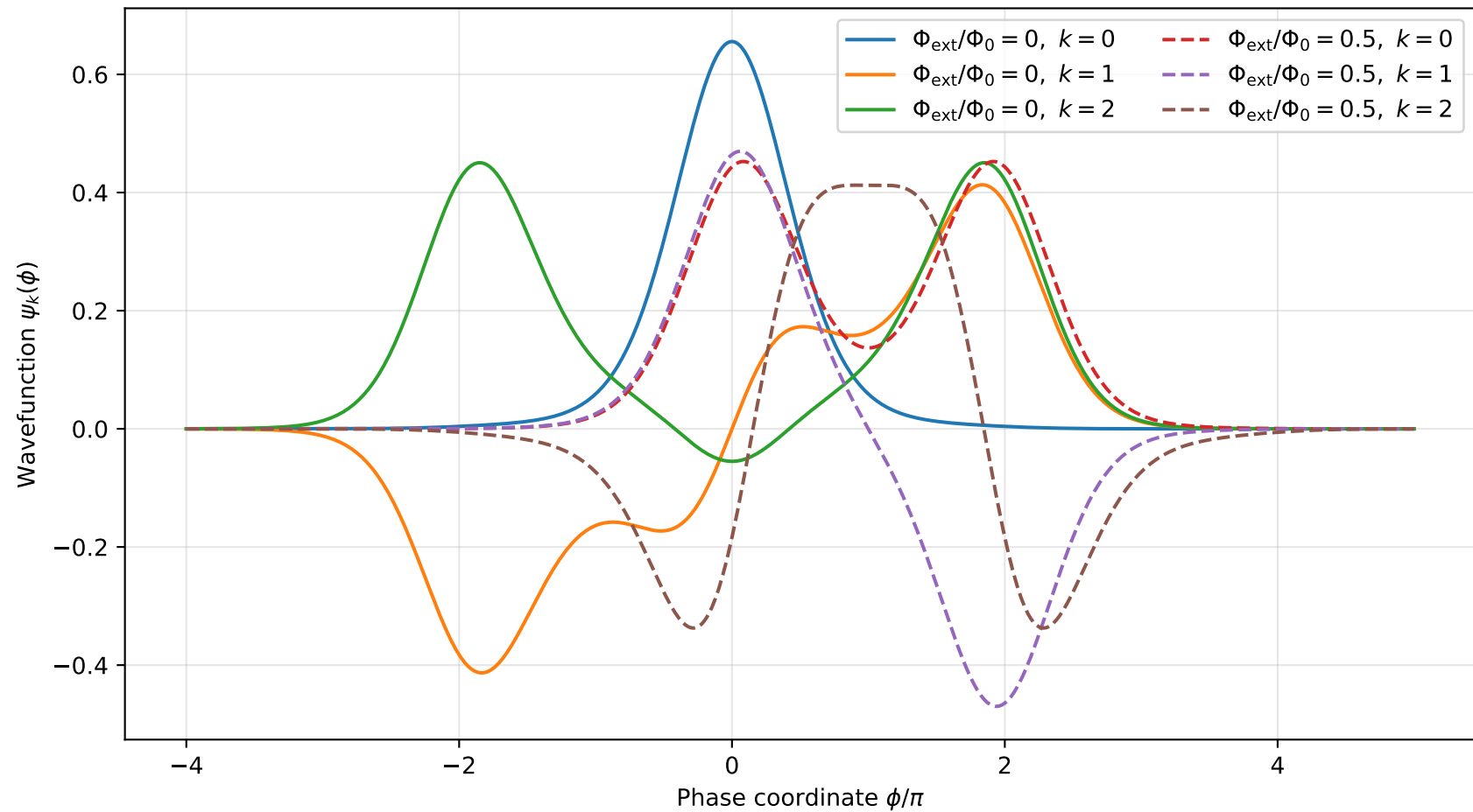
Selected fluxonium eigenfunctions solid: zero flux; dashed: half flux
