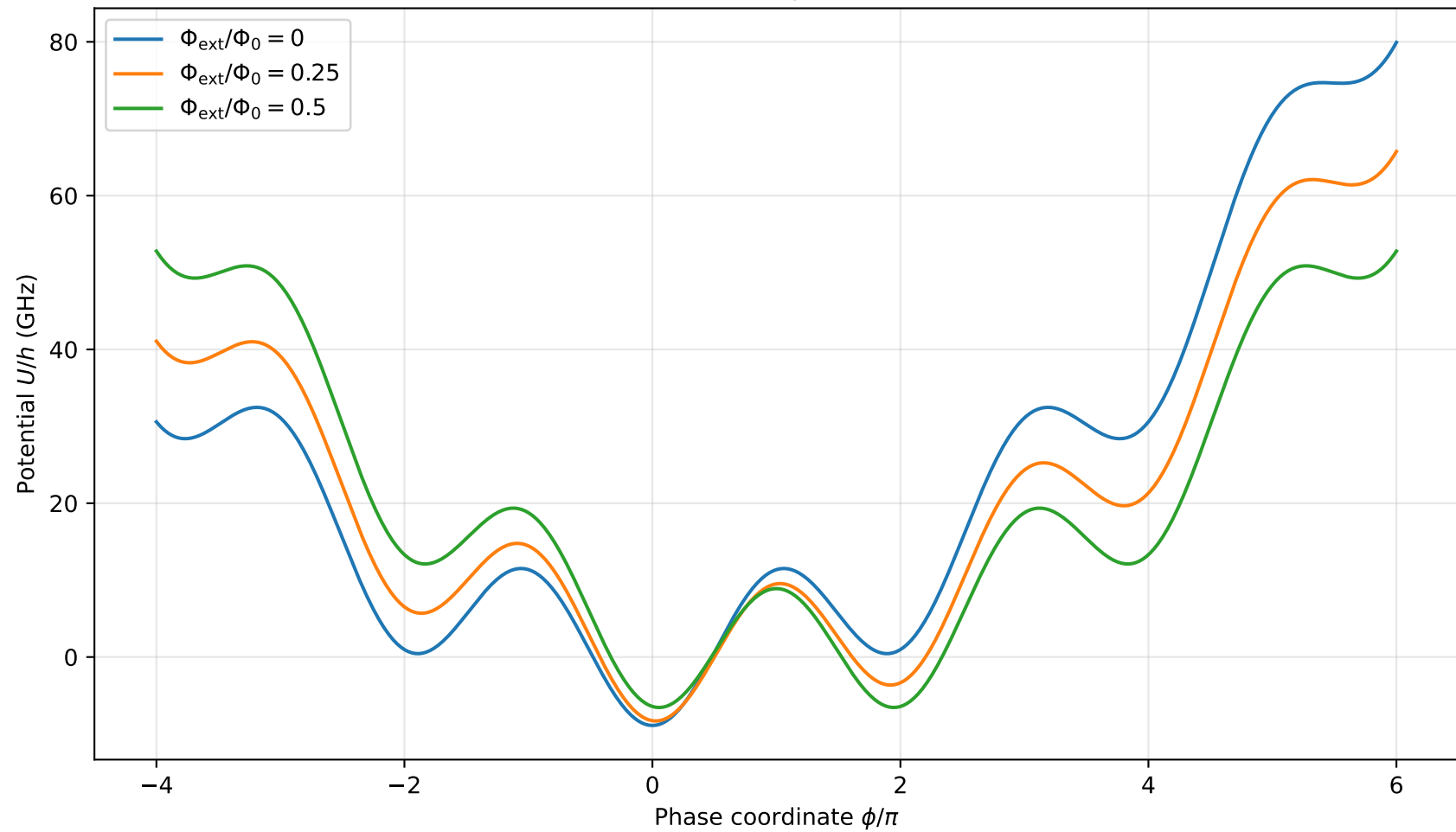
Fluxonium potential
