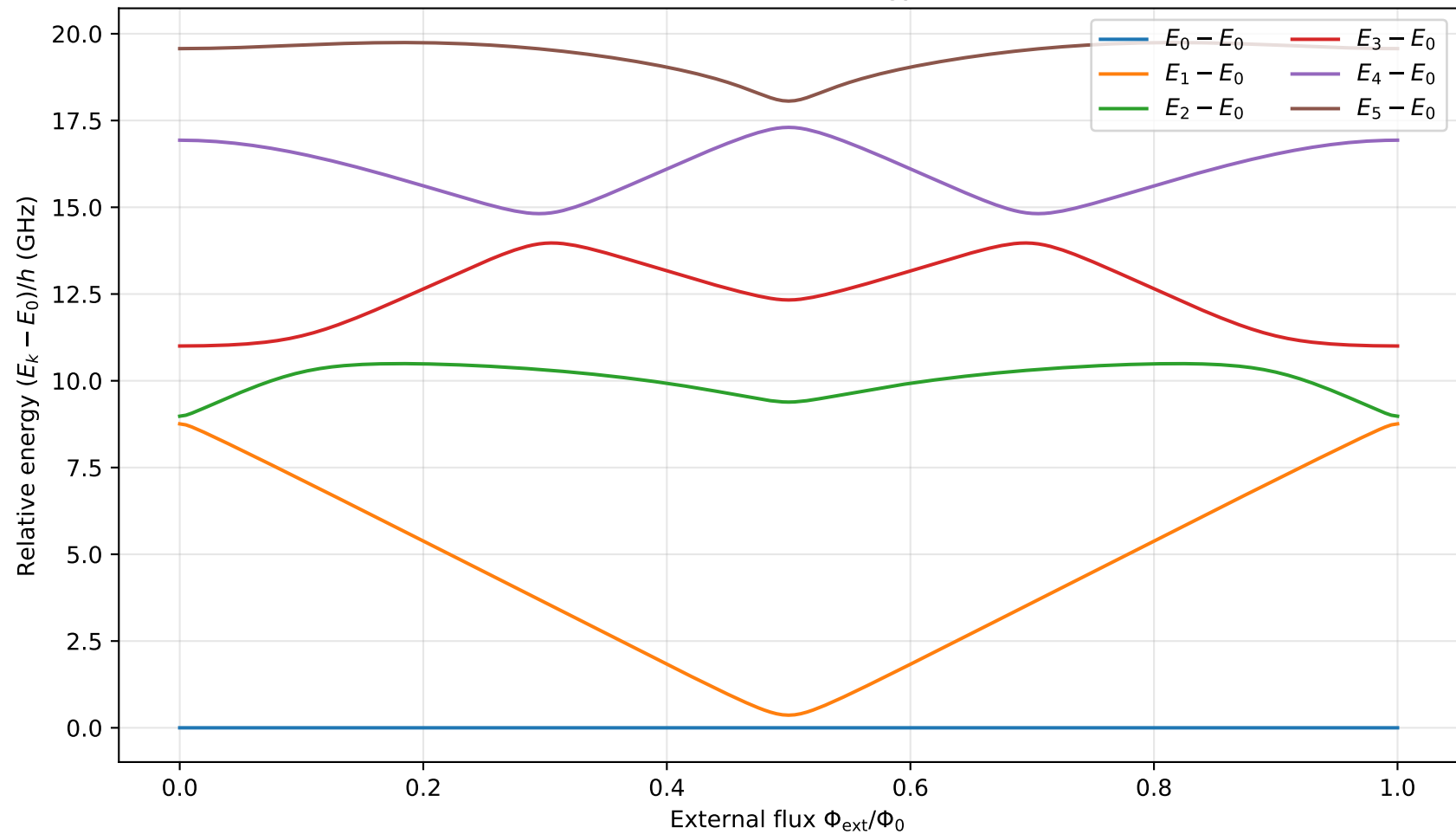
Lowest fluxonium energy levels
