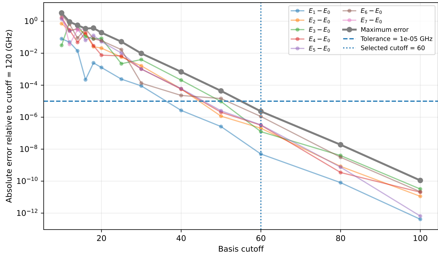
Convergence of Fluxonium Transition Energies at \Phi_{\text{ext}}/\Phi_0 = 0.5
