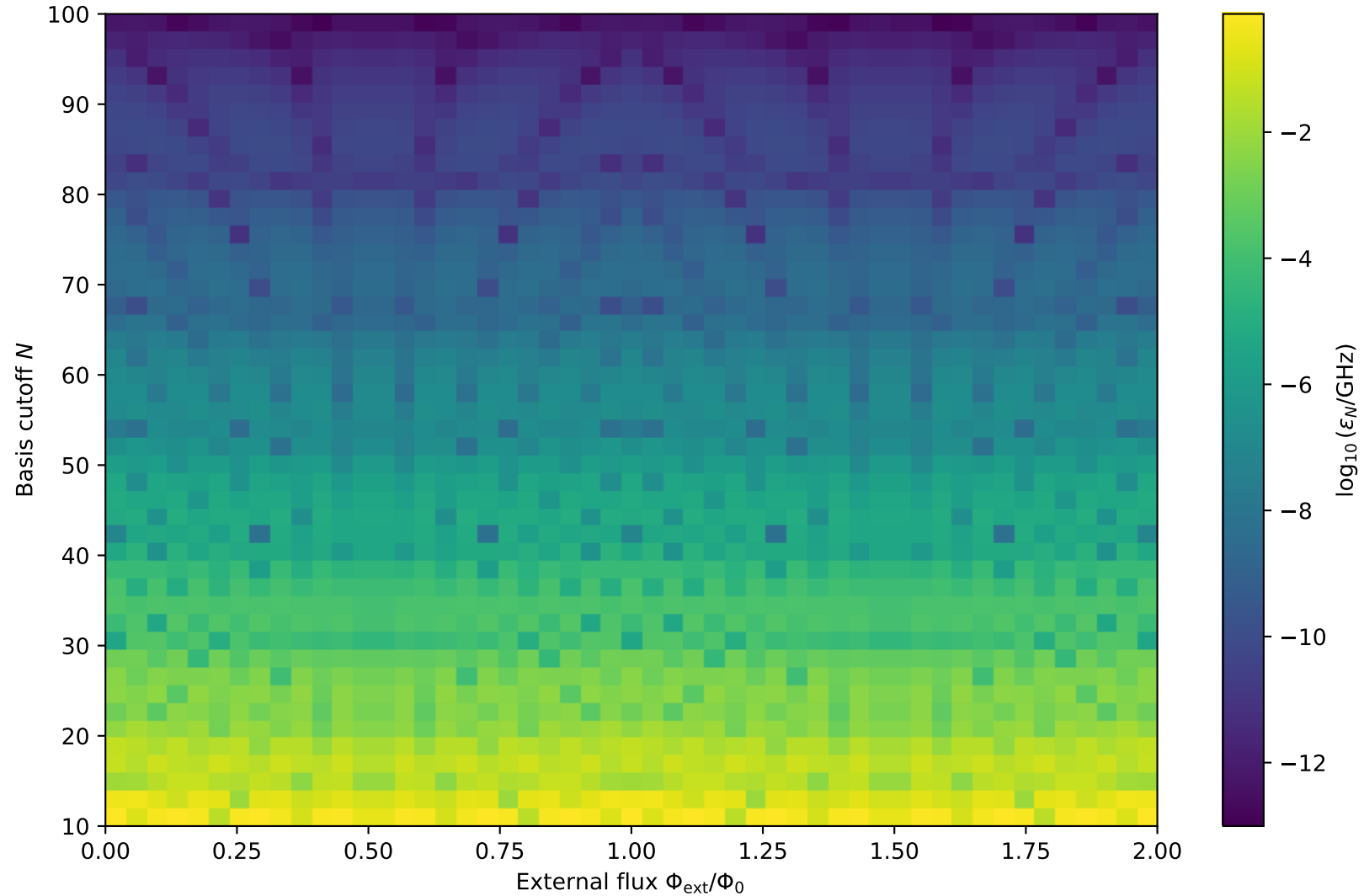
Basis-truncation error in the 0 \rightarrow 1 transition
