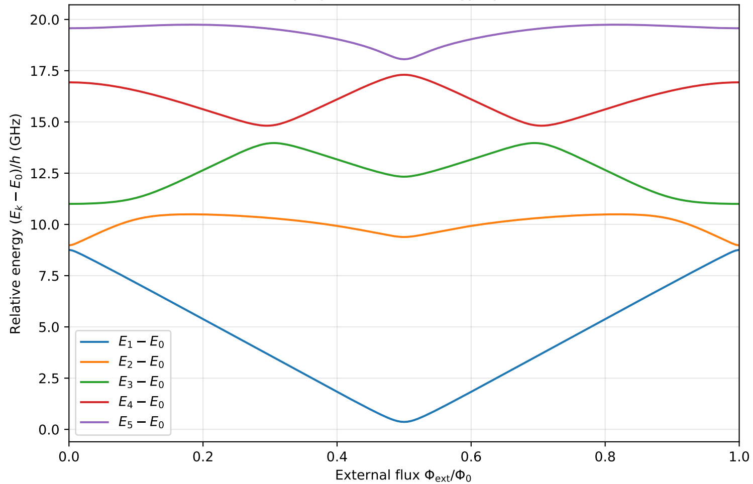
Low-Lying Fluxonium Energy Spectrum
