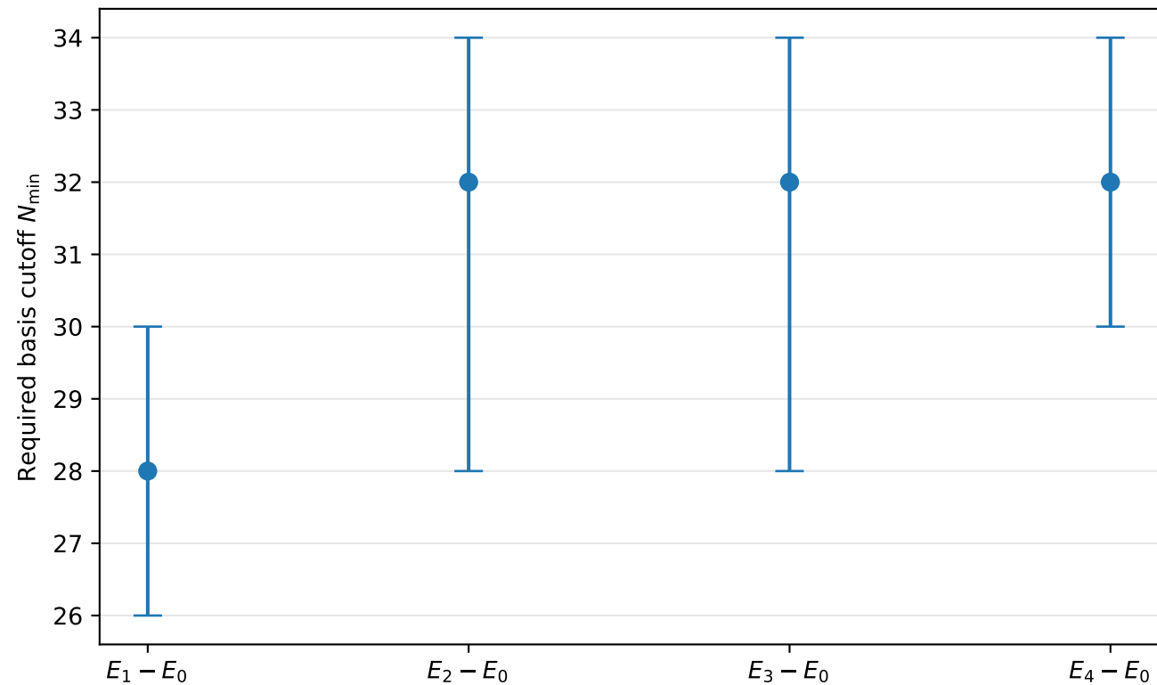
Basis cutoff required for 1 MHz accuracy
