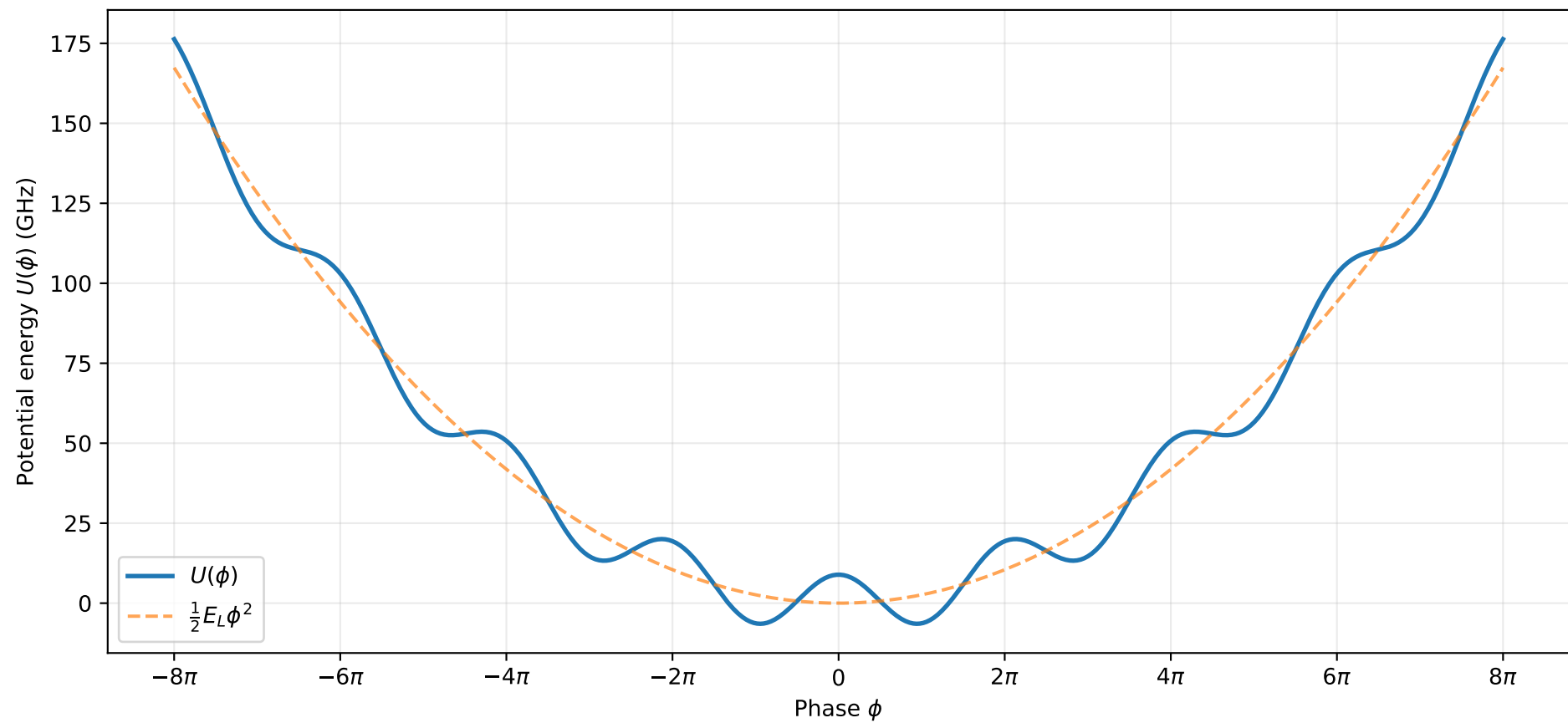
Fluxonium Potential at \Phi_{\text{ext}}/\Phi_0 = 0.5
