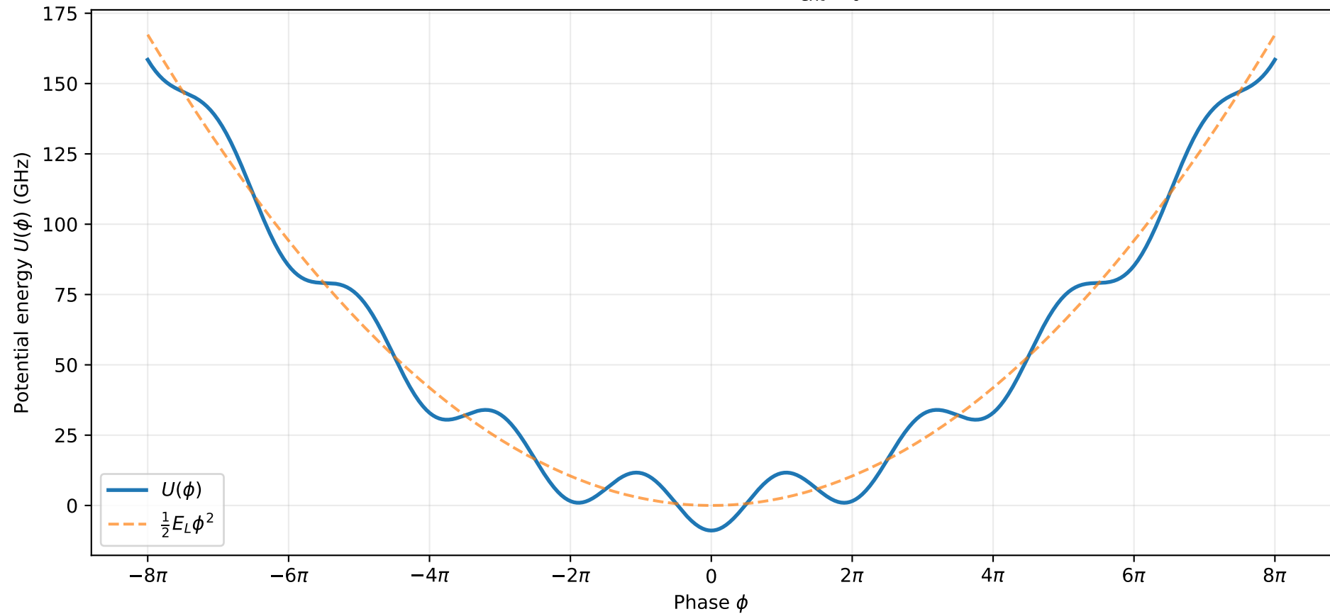
Fluxonium Potential at \Phi_{\text{ext}}/\Phi_0 = 0
