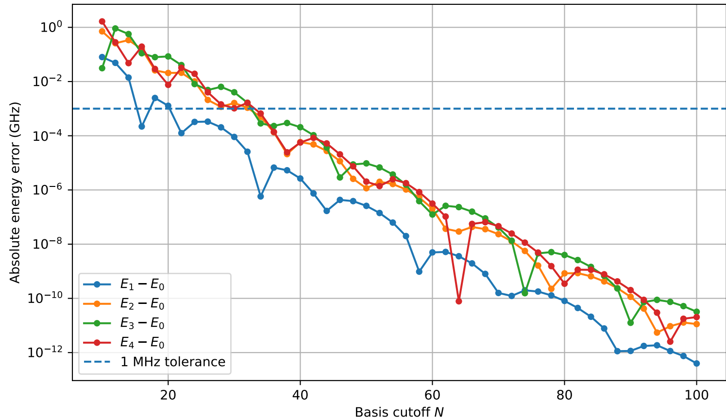
State-dependent convergence at \Phi_{\text{ext}}/\Phi_0 = 0.5
