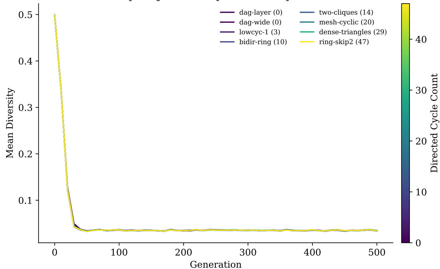
Diversity Trajectories by Directed Cycle Count
