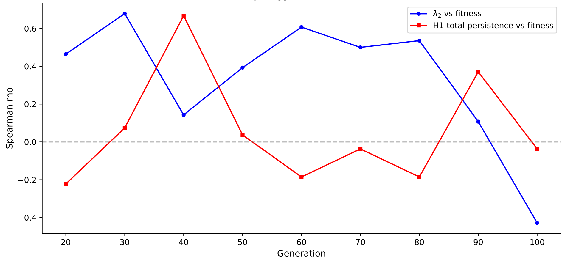
Correlation Between Topology Metrics and GA Fitness Over Time
