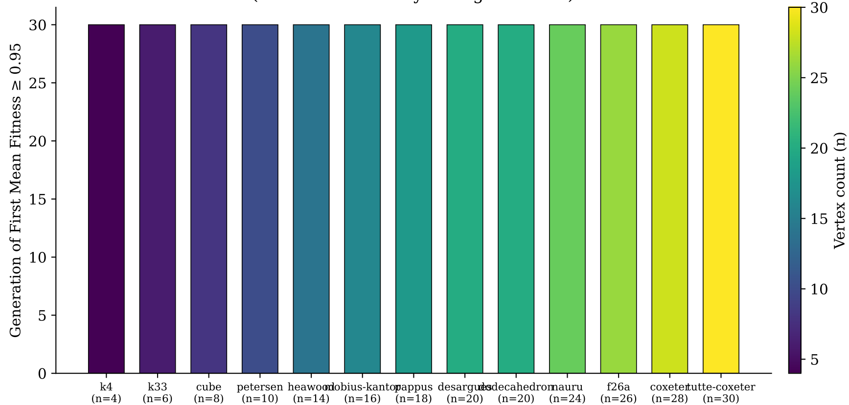
Convergence Speed by Topology (* = not reached by final generation)
