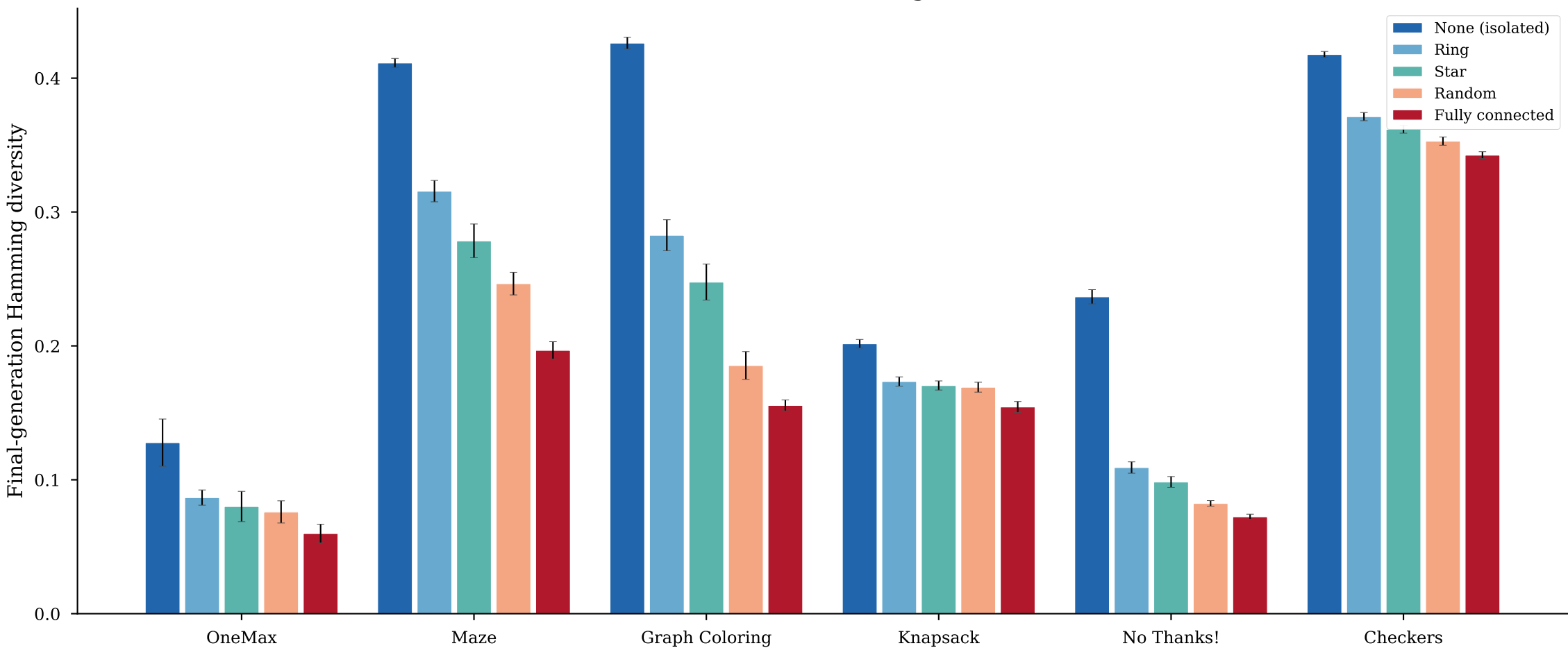
Multi-Domain Topology Ordering (6 domains) (mean \pm SE across 30 seeds, generation 99)
