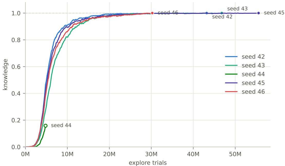
MPX-135 knowledge acquisition (pyalcs, acs2, GA true)
