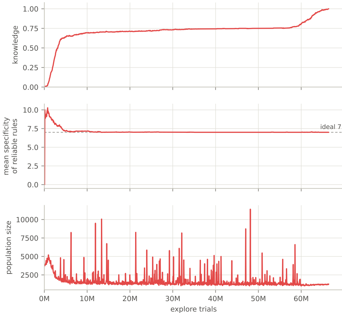
MPX-70 seed 46: knowledge, rule specificity and population size
