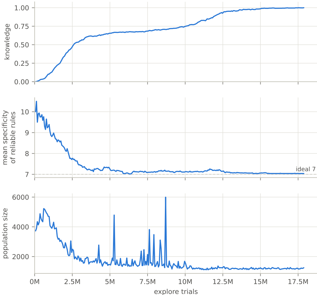
MPX-70 seed 42: knowledge, rule specificity and population size
