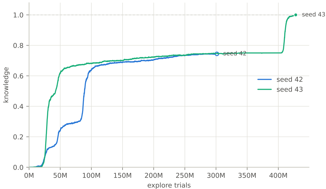
MPX-135 knowledge acquisition (pyalcs variant, GA on)
