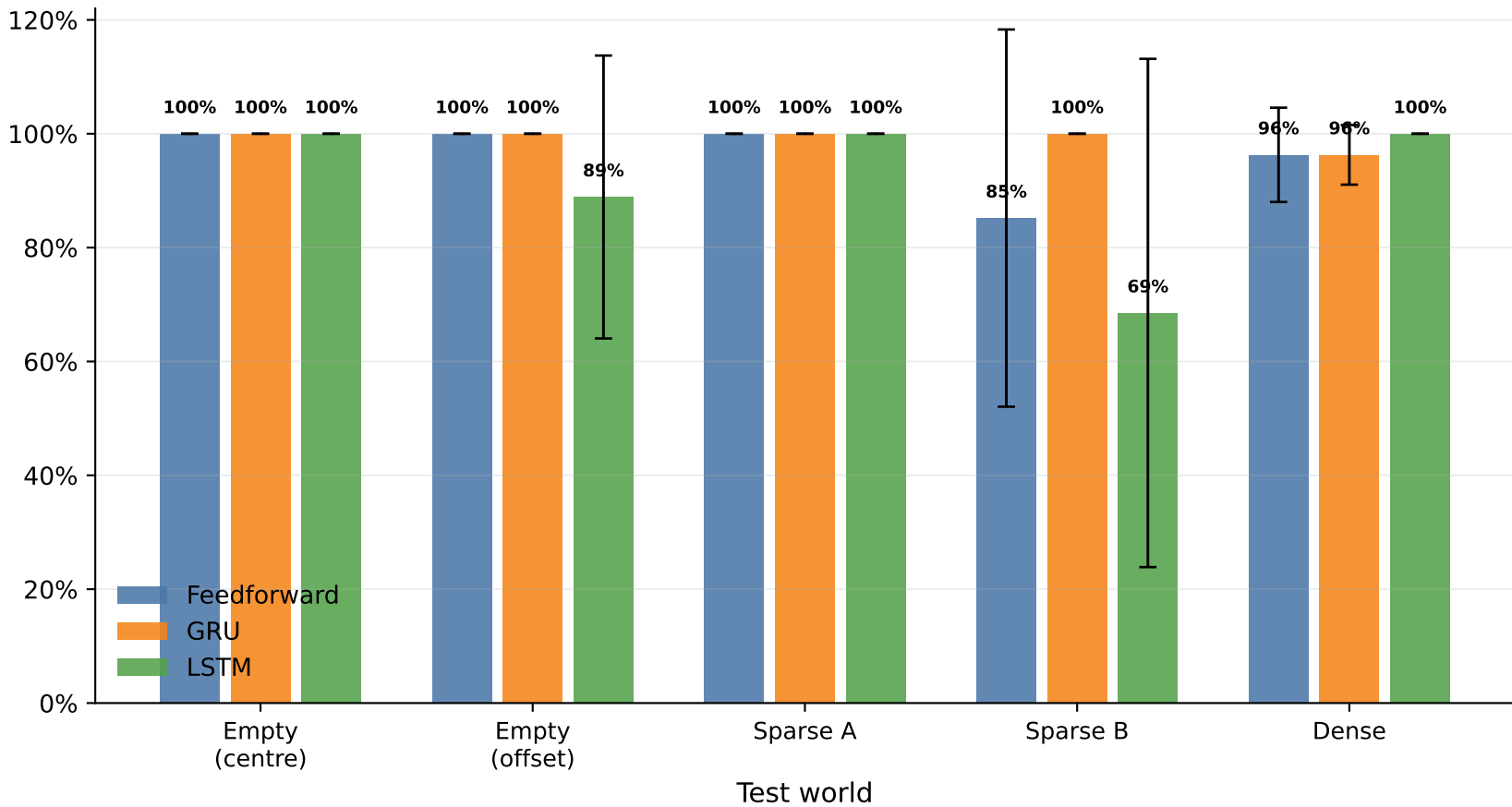
Success rate (9 episodes x 6 seeds)
