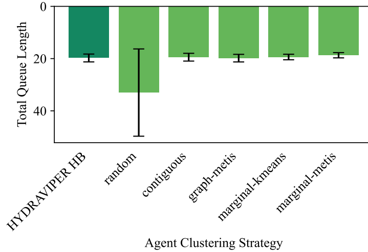
Figure 7.6: Performance of HYDRAVIPER on the Ingolstadt corridor (IC) under different agent set partitioning methods at the high budget level. graph-metis applies METIS to the environment graph; marginal-kmeans applies k -means clustering to pairwise Q -values; and marginal-metis applies METIS to the same.
