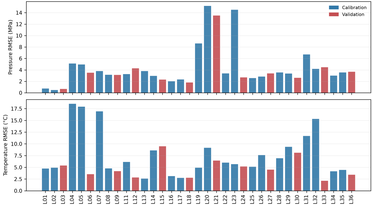
Figure 2: Case-level pressure and gas-temperature RMSE. The frozen validation cases are every third laboratory test; L10 was excluded by the pre-model mass-closure screen and therefore has no bar.
