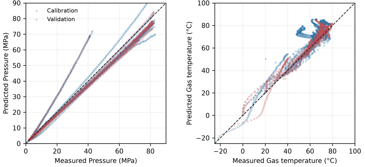
Figure 1: Measured and predicted tank pressure and gas temperature on the experimental time bases. Points are semi-transparent so repeated trajectories remain visible. The dashed line denotes equality.
