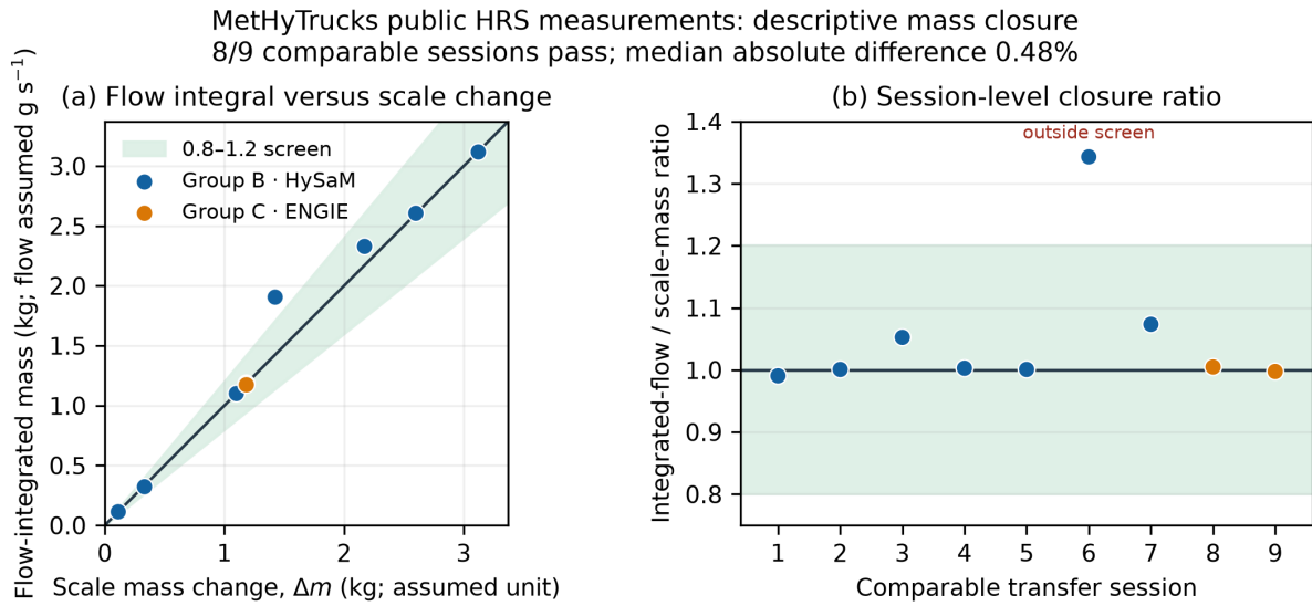
Figure 3: Descriptive flow/scale closure for nine MetHyTrucks sessions; workbook units remain audit assumptions.
