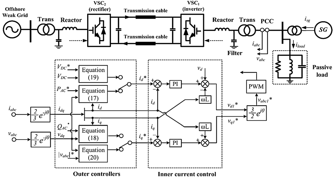
Fig. 1. Single-line diagram of VSC-HVDC transmission system, with the conventional control system.
