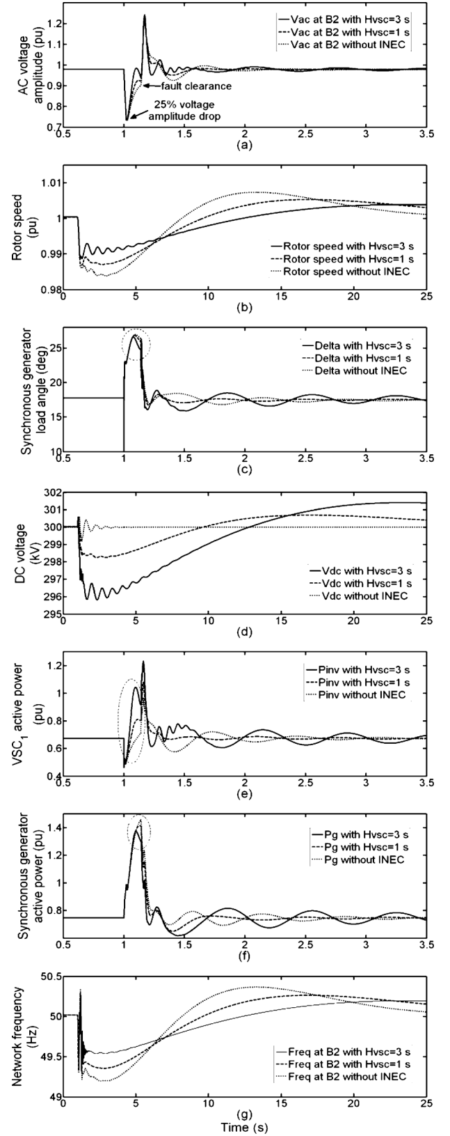
Fig. 11. INEC response for 140-ms three-phase-to-ground distant fault: (a) zoomed AC voltage amplitude at B 2 ; (b) SG rotor speed; (c) zoomed SG load angle; (d) HVDC DC link voltage; (e) zoomed VSC 1 active power; (f) zoomed SG active power; (g) Network frequency.
