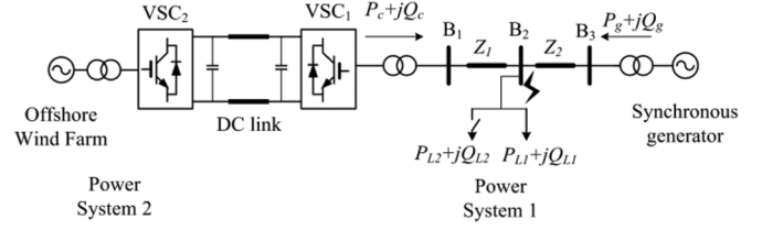
Fig. 5. Single-line diagram of the simulated test system.
