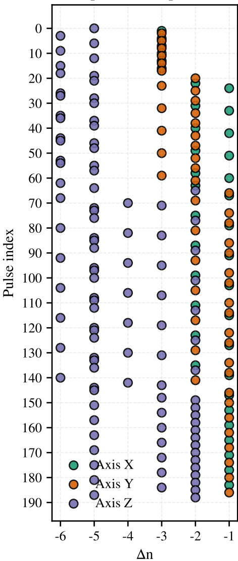
Optimized sequence
