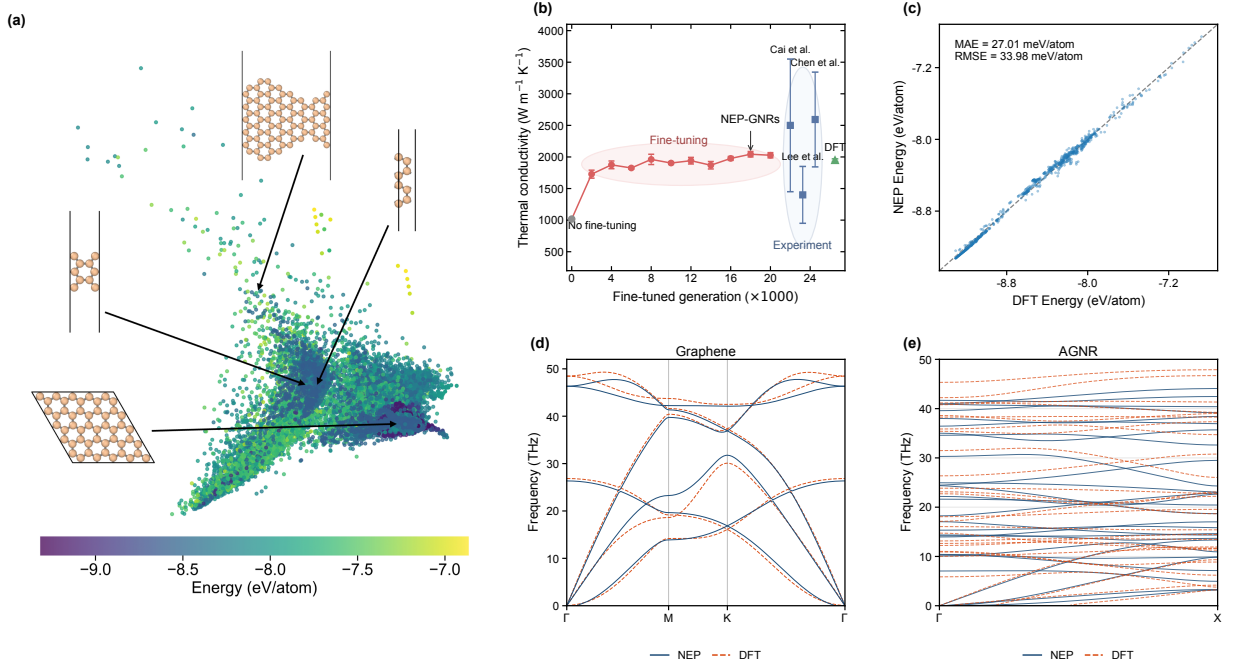
FIG. 1. Validation of the fine-tuned NEP-GNRs potential for graphene and graphene-nanoribbon edge environments. (a) Principal component analysis projection of the atomic descriptors in the fine-tuning dataset. (b) Evolution of the predicted thermal conductivity of pristine graphene at 300 K during fine-tuning from the pretrained NEP89 model to NEP-GNRs, together with representative DFT and experimental values reported in the literature [43–45]. (c) Parity plot comparing the energies predicted by NEP-GNRs with the corresponding DFT reference values. MAE and RMSE denote the mean absolute error and root-mean-square error, respectively. (d) Phonon dispersion of pristine graphene predicted by NEP-GNRs compared with the reference DFT result along the \Gamma -M-K- \Gamma path. (e) Phonon dispersion of a representative armchair graphene nanoribbon predicted by NEP-GNRs compared with the DFT reference result along the \Gamma -X path.
