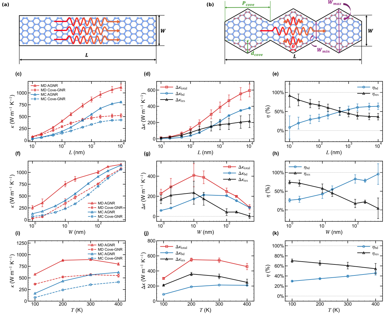
FIG. 2. Atomic structures and size- and temperature-dependent thermal-transport suppression in graphene nanoribbons with different edge morphologies. (a) Pristine AGNR with unpassivated straight armchair edges. (b) Cove-GNR with unpassivated periodically modulated edges. Here, P_{\text{cove}} denotes the cove period, d_{\text{cove}} denotes the cove depth, W_{\text{min}} and W_{\text{max}} denote the minimum and maximum transverse distances between the two opposing edges, respectively, and \theta denotes the local vertex angle associated with the cove modulation. The effective ribbon width is defined as W = (W_{\text{min}} + W_{\text{max}})/2 , and the AGNR and Cove-GNR are compared at the same W . (c) Length-dependent thermal conductivity \kappa at a fixed width of W = 20 nm obtained from MD-based spectral reconstruction and phonon MC simulations. (d) Length-dependent comparison of the total MD reduction \Delta\kappa_{\text{total}} , the boundary reduction predicted by the semiclassical MC model \Delta\kappa_{\text{bd}} , and the resulting effective atomistic residual \Delta\kappa_{\text{res}} . (e) Corresponding normalized model terms \eta_{\text{bd}} and \eta_{\text{res}} as functions of length. (f) Width-dependent thermal conductivity at a fixed length of L = 1000 nm. (g) Corresponding width-dependent comparison of \Delta\kappa_{\text{total}} , \Delta\kappa_{\text{bd}} , and \Delta\kappa_{\text{res}} . (h) Normalized model terms \eta_{\text{bd}} and \eta_{\text{res}} as functions of width. (i) Temperature-dependent thermal conductivity at fixed ribbon dimensions of W = 50 nm and L = 1000 nm. (j) Temperature-dependent comparison of \Delta\kappa_{\text{total}} , \Delta\kappa_{\text{bd}} , and the effective atomistic residual \Delta\kappa_{\text{res}} . (k) Normalized model terms \eta_{\text{bd}} and \eta_{\text{res}} as functions of temperature. In panels (c), (f), and (i), red and blue curves denote the MD-based spectral reconstruction and MC results, respectively; solid triangle-marked lines correspond to pristine AGNRs, whereas dashed circle-marked lines correspond to Cove-GNRs.
