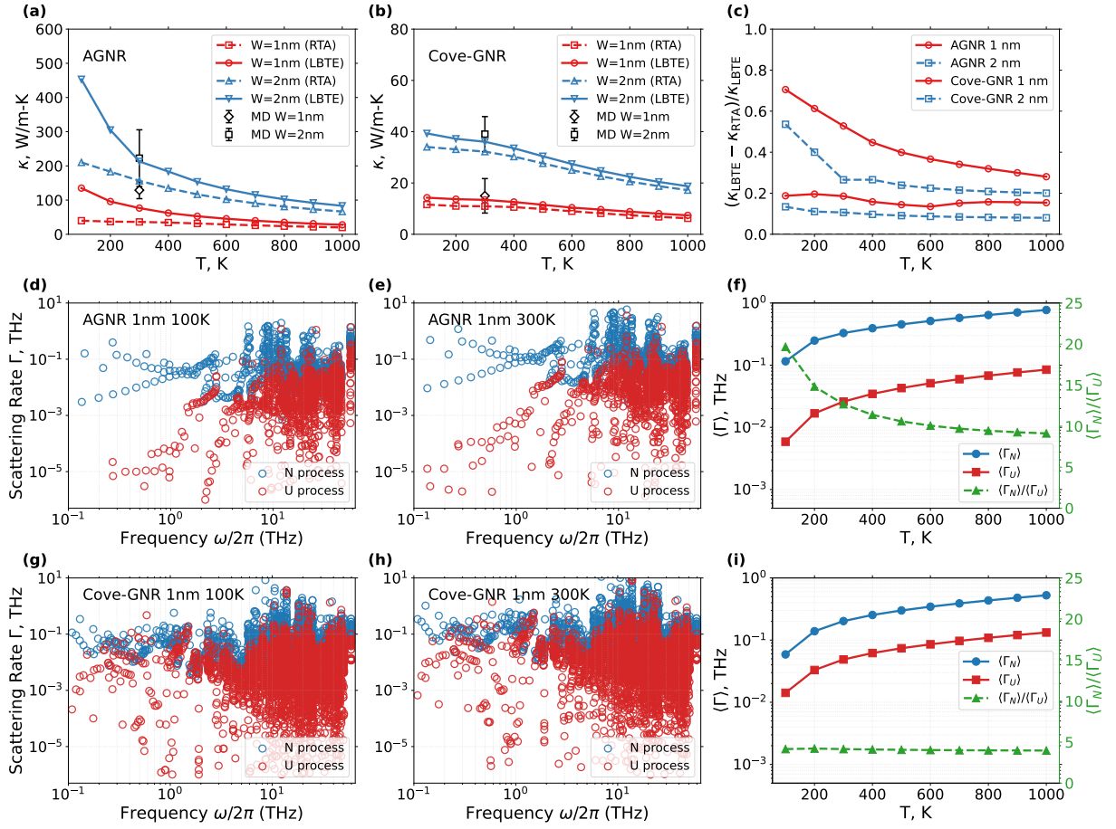
FIG. 4. Lattice thermal transport and Normal/Umklaup scattering in graphene nanoribbons with different edge geometries. (a,b) Temperature-dependent thermal conductivity \kappa of AGNRs and Cove-GNRs with widths of 1 and 2 nm, calculated using the relaxation-time approximation and the direct solution of the full linearized phonon Boltzmann transport equation. The black symbols in panels (a) and (b) denote MD-based thermal-conductivity values at 300 K for W = 1 and 2 nm, included for comparison with the LBTE/RTA results at overlapping ribbon widths. (c) Relative collective correction, \eta_c = (\kappa_{\text{LBTE}} - \kappa_{\text{RTA}})/\kappa_{\text{LBTE}} , quantifying the mode-to-mode coupling correction beyond the independent-mode RTA description. (d,e) Mode-resolved frequency-dependent Normal ( N ) and Umklapp ( U ) three-phonon scattering rates in the 1-nm-wide AGNR at 100 and 300 K, respectively. (f) Transport-weighted average scattering rates \langle \Gamma_N \rangle and \langle \Gamma_U \rangle , together with the ratio \langle \Gamma_N \rangle / \langle \Gamma_U \rangle , for the 1-nm-wide AGNR. (g,h) Corresponding mode-resolved frequency-dependent N and U scattering rates in the 1-nm-wide Cove-GNR at 100 and 300 K, respectively. (i) Transport-weighted average scattering rates and their ratio for the 1-nm-wide Cove-GNR.
