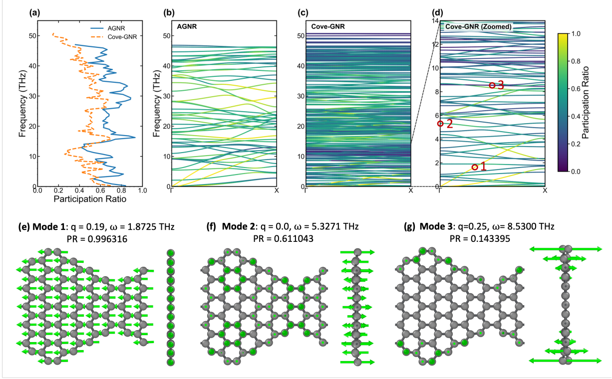
FIG. 3. Participation-ratio analysis and representative phonon eigenmodes of the AGNR and Cove-GNR. (a) Frequency-resolved average participation ratios of phonon modes in the two nanoribbons. Smaller values indicate stronger spatial confinement of the atomic displacements within the unit cell. (b) Phonon dispersion of the AGNR colored by the mode participation ratio. (c) Phonon dispersion of the Cove-GNR colored by the mode participation ratio. (d) Enlarged low-frequency region of the Cove-GNR dispersion. Red circles identify three representative modes selected for real-space eigenvector visualization. (e) Representative extended mode in the Cove-GNR at the reduced wave-vector coordinate q = 0.19 , with \omega/2\pi = 1.8725 THz and PR = 0.996316 . (f) Representative partially confined mode at the \Gamma point, with q = 0 , \omega/2\pi = 5.3271 THz and PR = 0.611043 . (g) Representative strongly edge-confined mode at q = 0.25 , with \omega/2\pi = 8.5300 THz and PR = 0.143395 . Green arrows represent the atomic displacement vectors. The color scale in panels (b)–(d) denotes the participation ratio, with larger values corresponding to spatially extended modes and smaller values corresponding to increasingly confined modes.
