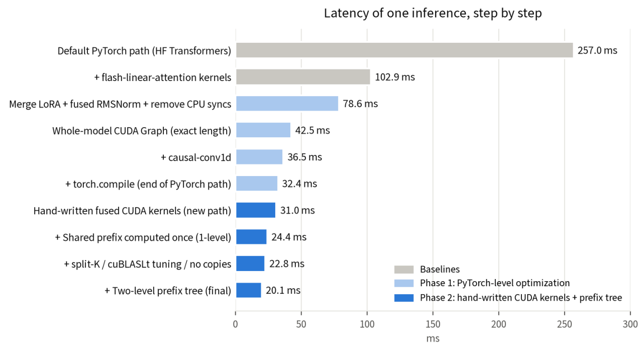
Figure 1. Latency of one inference on the example request as optimizations are added. Phase 1 works at the PyTorch level; phase 2 replaces the phase-1 path with hand-written CUDA kernels plus a prefix tree. Each bar is the median latency (ms) of the forward pass plus scoring head on one B300. The first two bars and the last bar were measured together with one script (bench/e2e_bench.py); the middle bars were measured during development.
