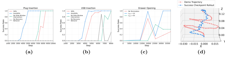
Fig. 6: Ablation study and trajectory comparison: (a) and (b) results on the plug insertion and USB insertion tasks under the No sliding window intervention and No recovery mechanism settings, respectively. (c) results on the drawer opening task under the No intervention termination setting. (d) results on 3D visualization of the demo trajectory and the policy rollout trajectory trained from it for the plug insertion task.
