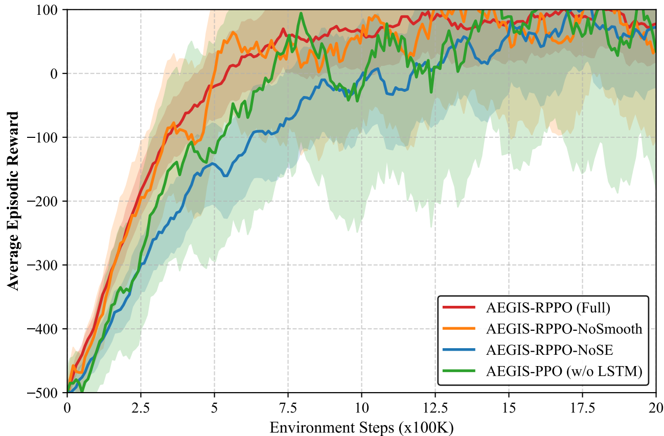
Training Convergence across Ablation Variants
