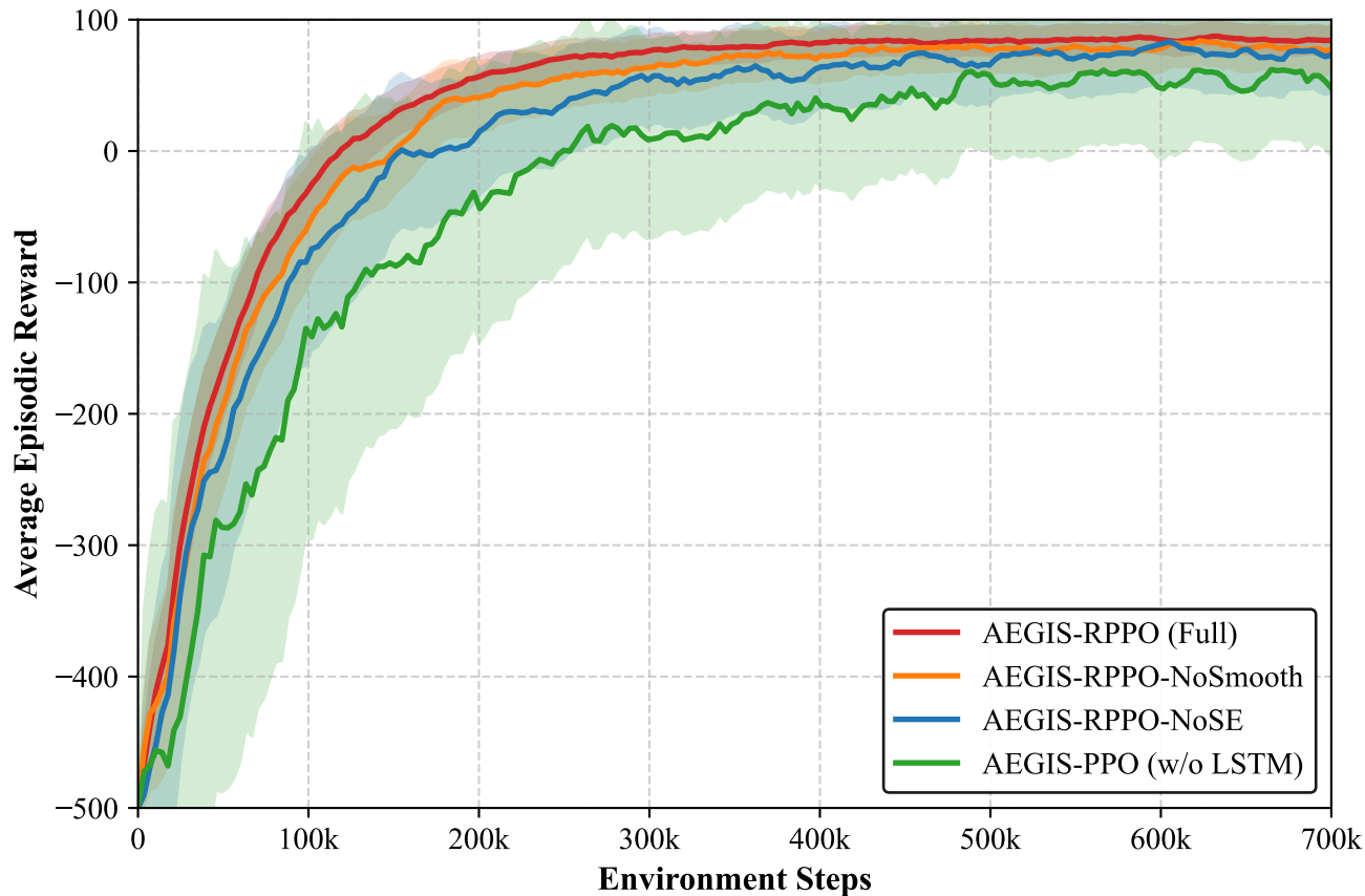
Training Convergence across Ablation Variants
