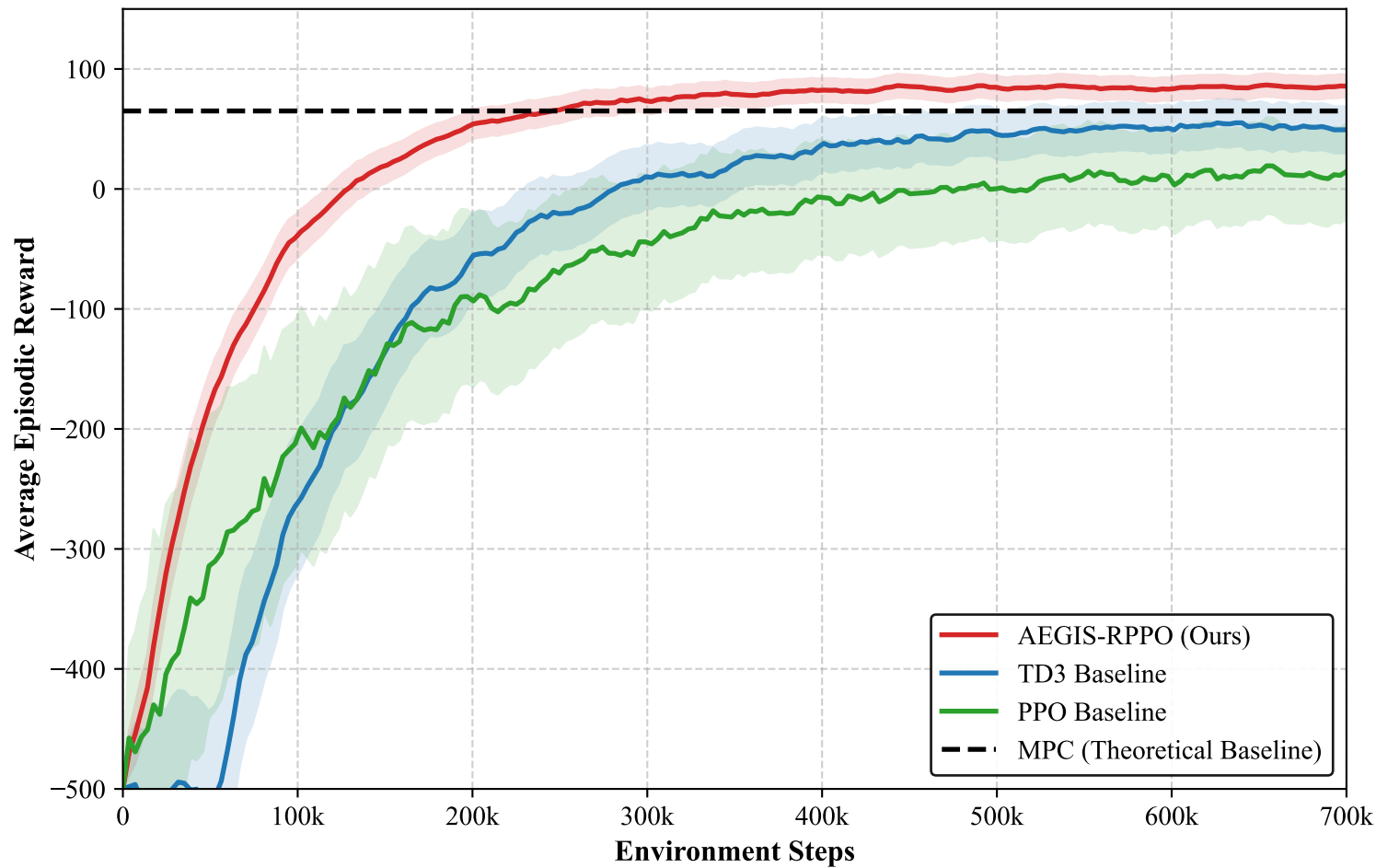
Training Convergence Comparison against Baselines
