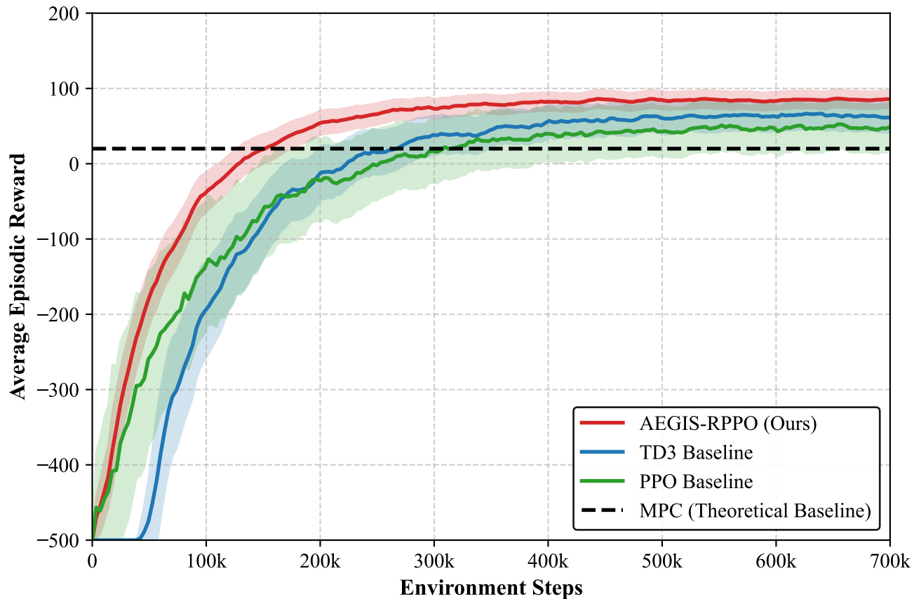
Training Convergence against Baselines
