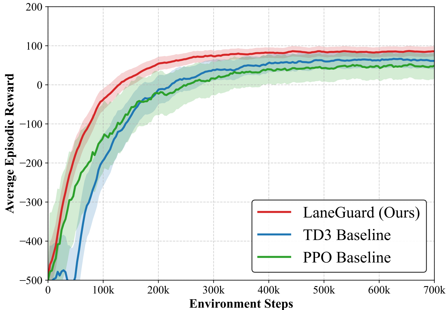
Training Convergence against Baselines
