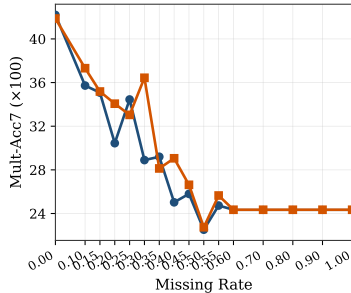
(a) Mult-Acc7
