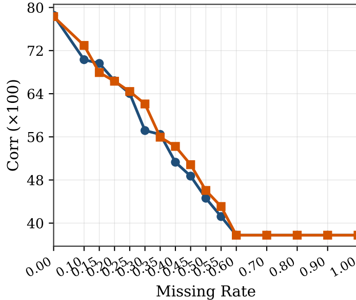
(b) Correlation
