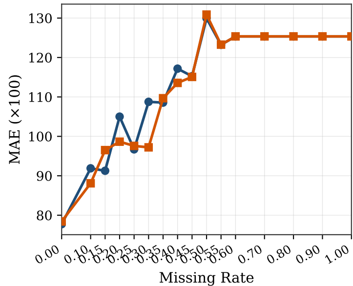
(c) MAE
