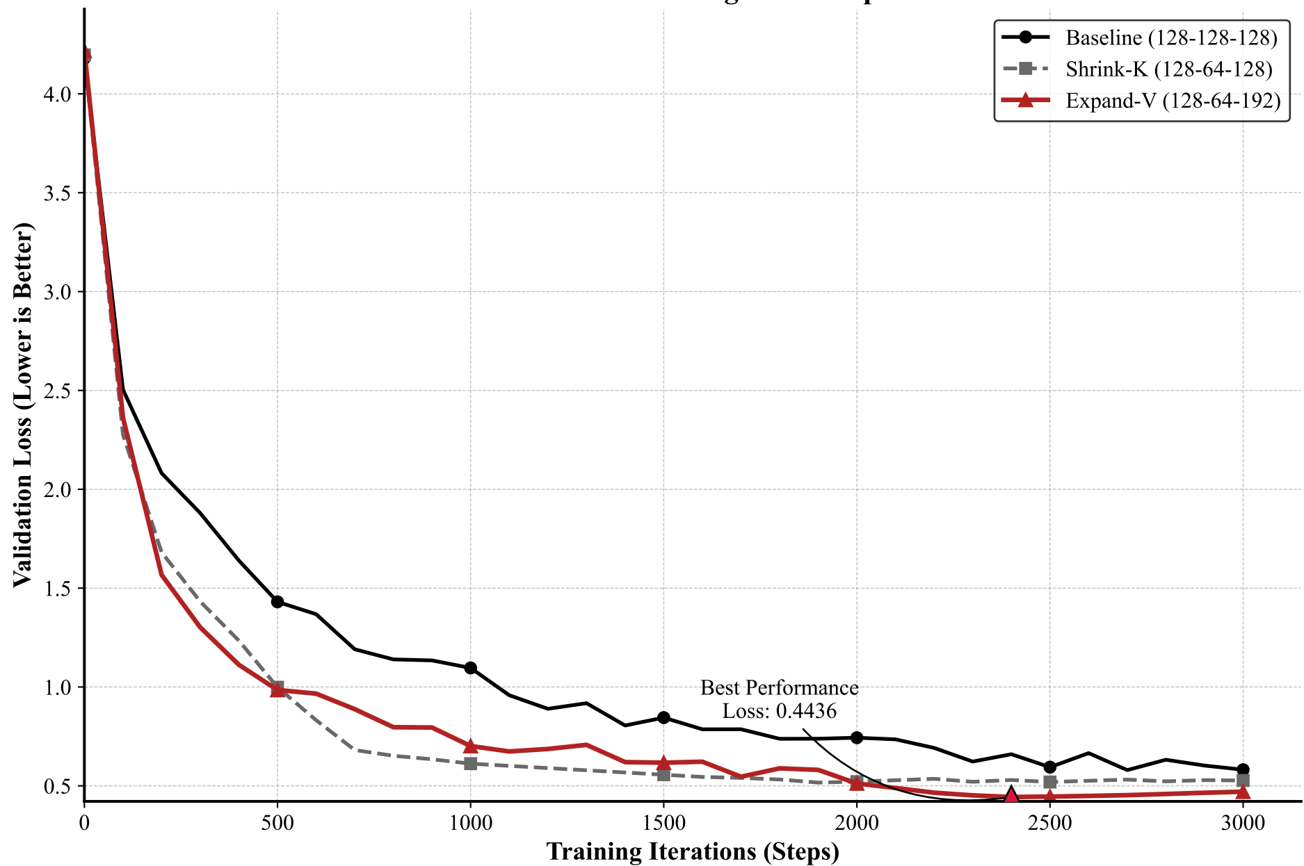
Validation Loss Convergence Comparison
