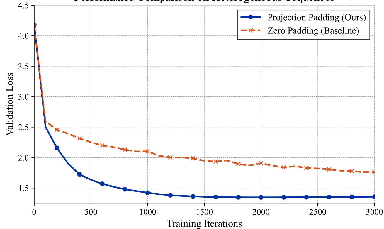
Performance Comparison on Heterogeneous Sequences
