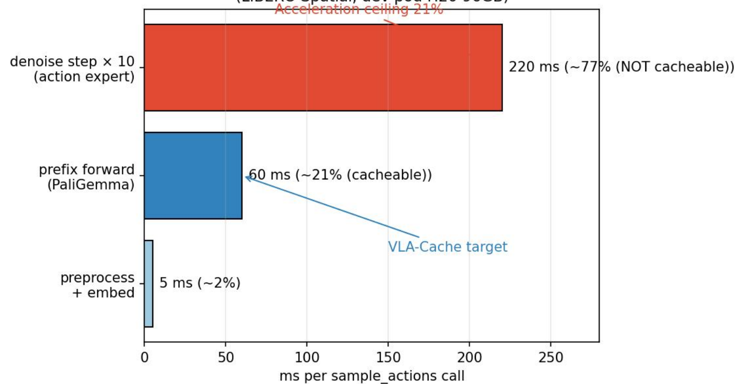
\pi 0.5 inference latency breakdown (LIBERO Spatial, dev pod H20 96GB)
