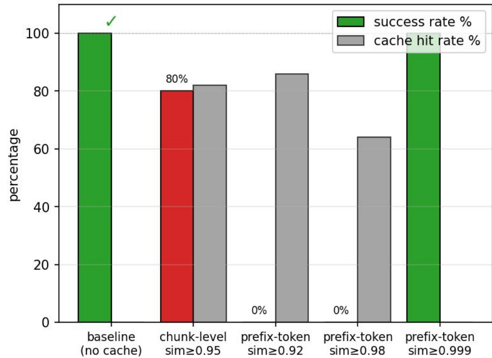
KV-Cache strategy benchmark on LIBERO Spatial \times \pi 0.5 (success rate vs cache hit rate)
