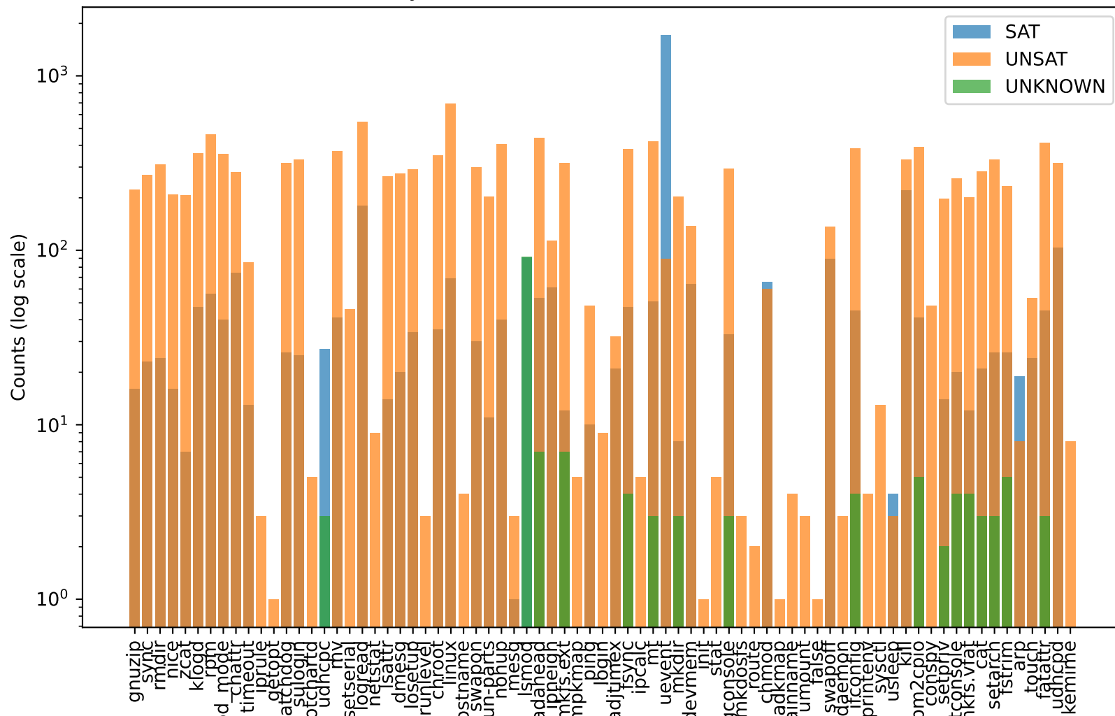
busybox - SAT, UNSAT, UNKNOWN Counts
