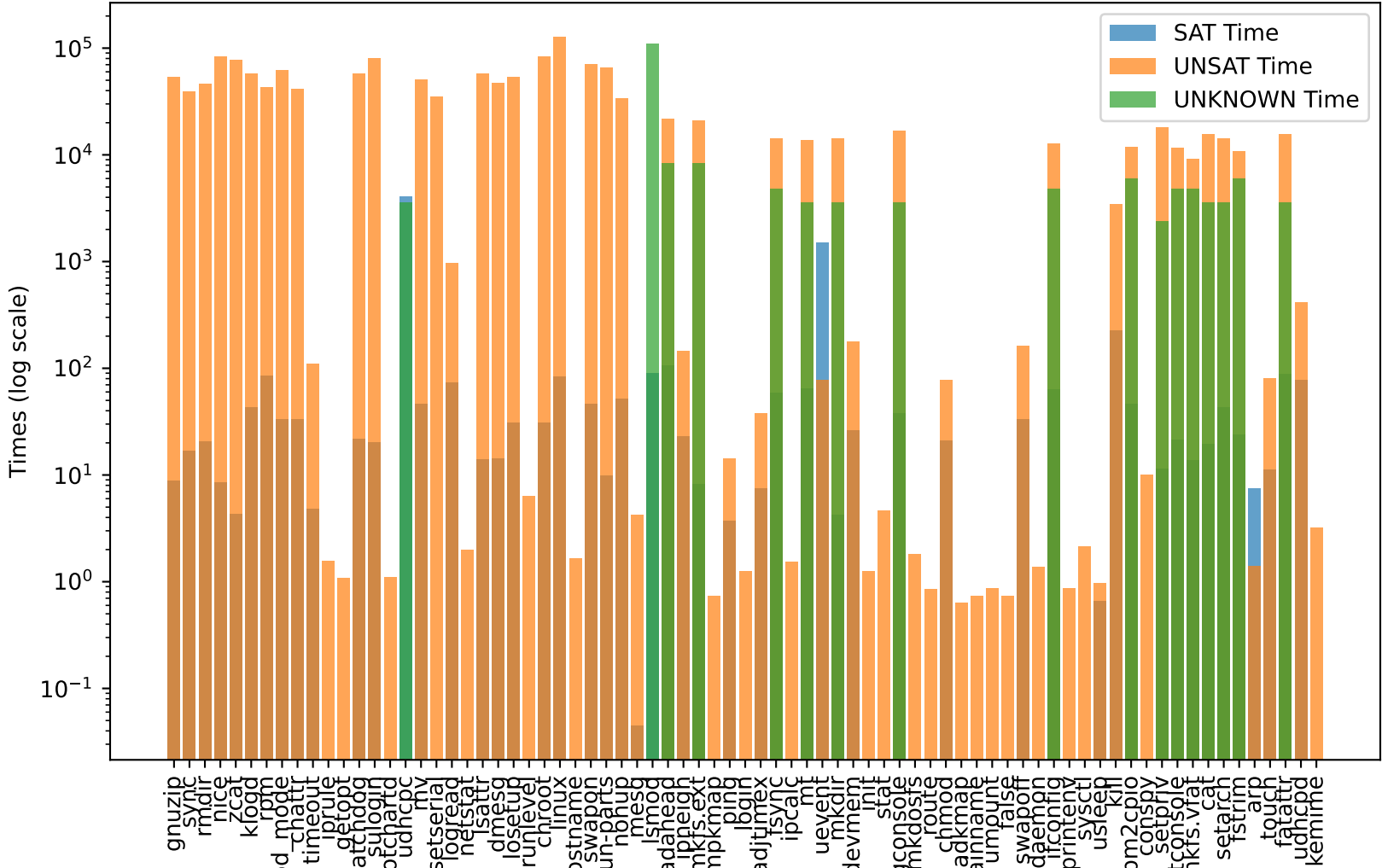
busybox - SAT, UNSAT, UNKNOWN Times
