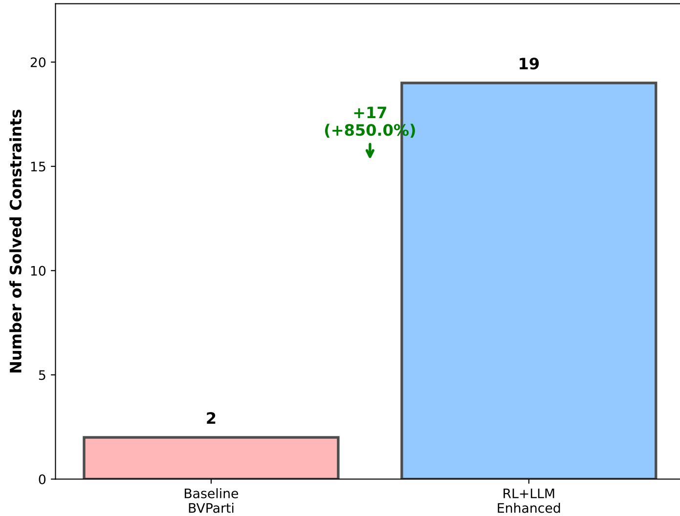
BVParti: Solving Capability Comparison
