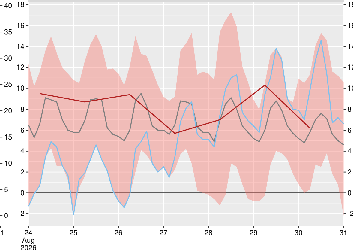
Ловеч (15525), 2026-08-30 06:00:00
