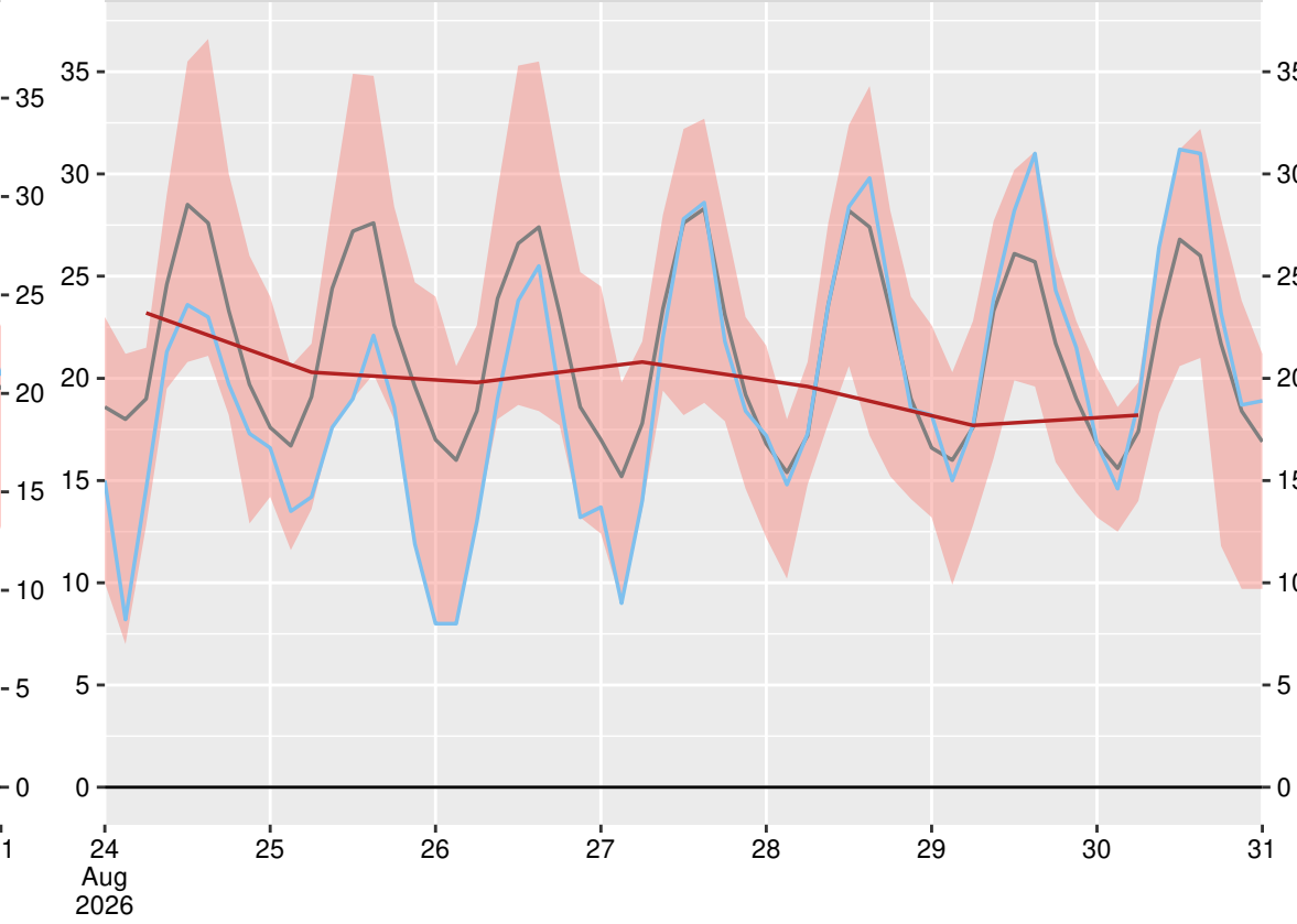
София (15614), 2026-08-30 06:00:00
