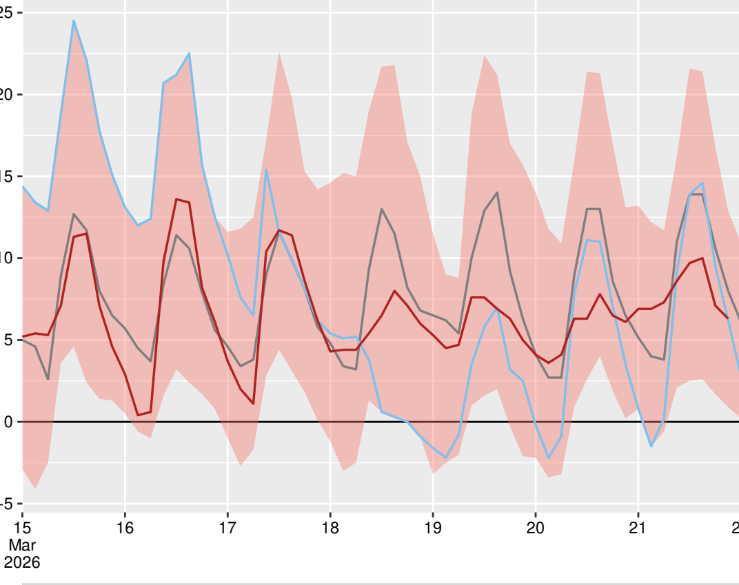
Разград (15549), 2026-03-21 21:00:00
