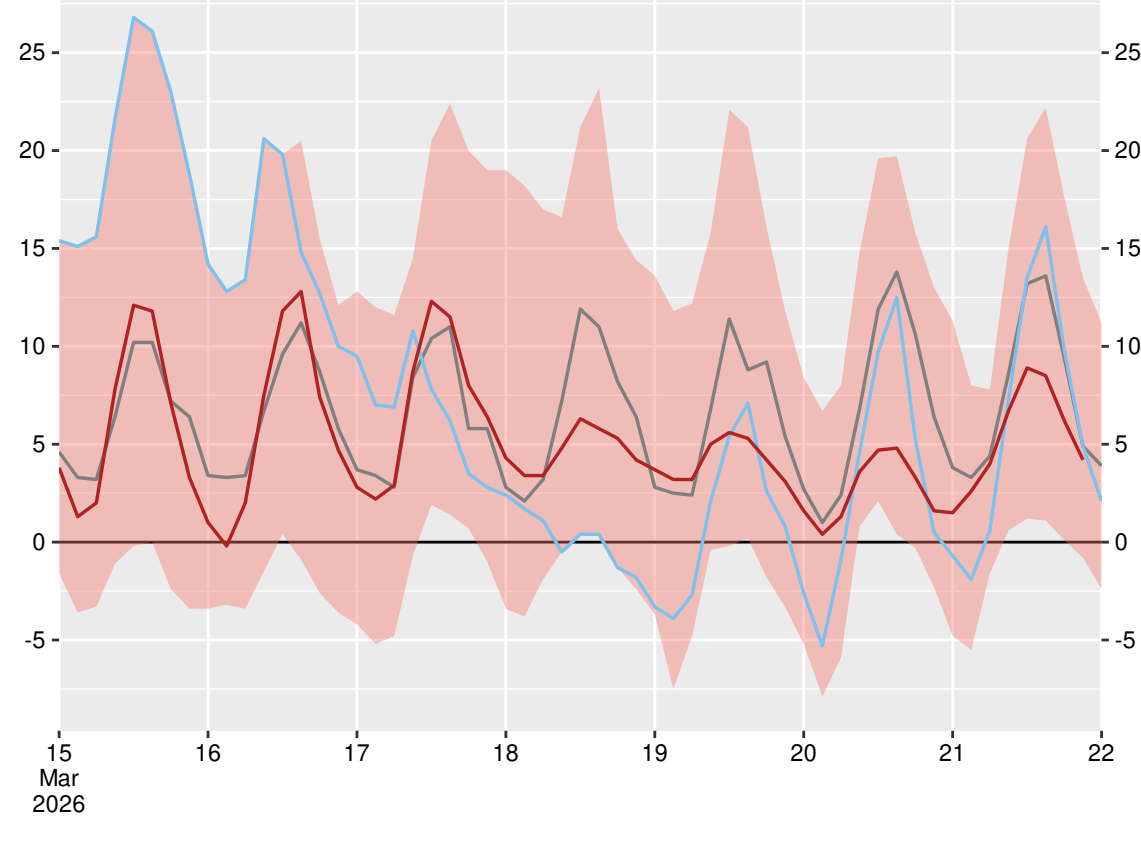
София (15614), 2026-03-21 21:00:00
