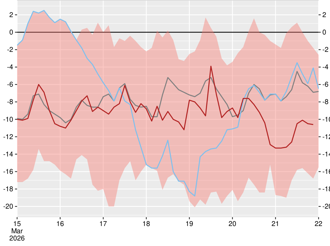
Ловеч (15525), 2026-03-21 21:00:00
